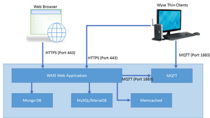
Figure 1. Wyse Management Suite architecture
