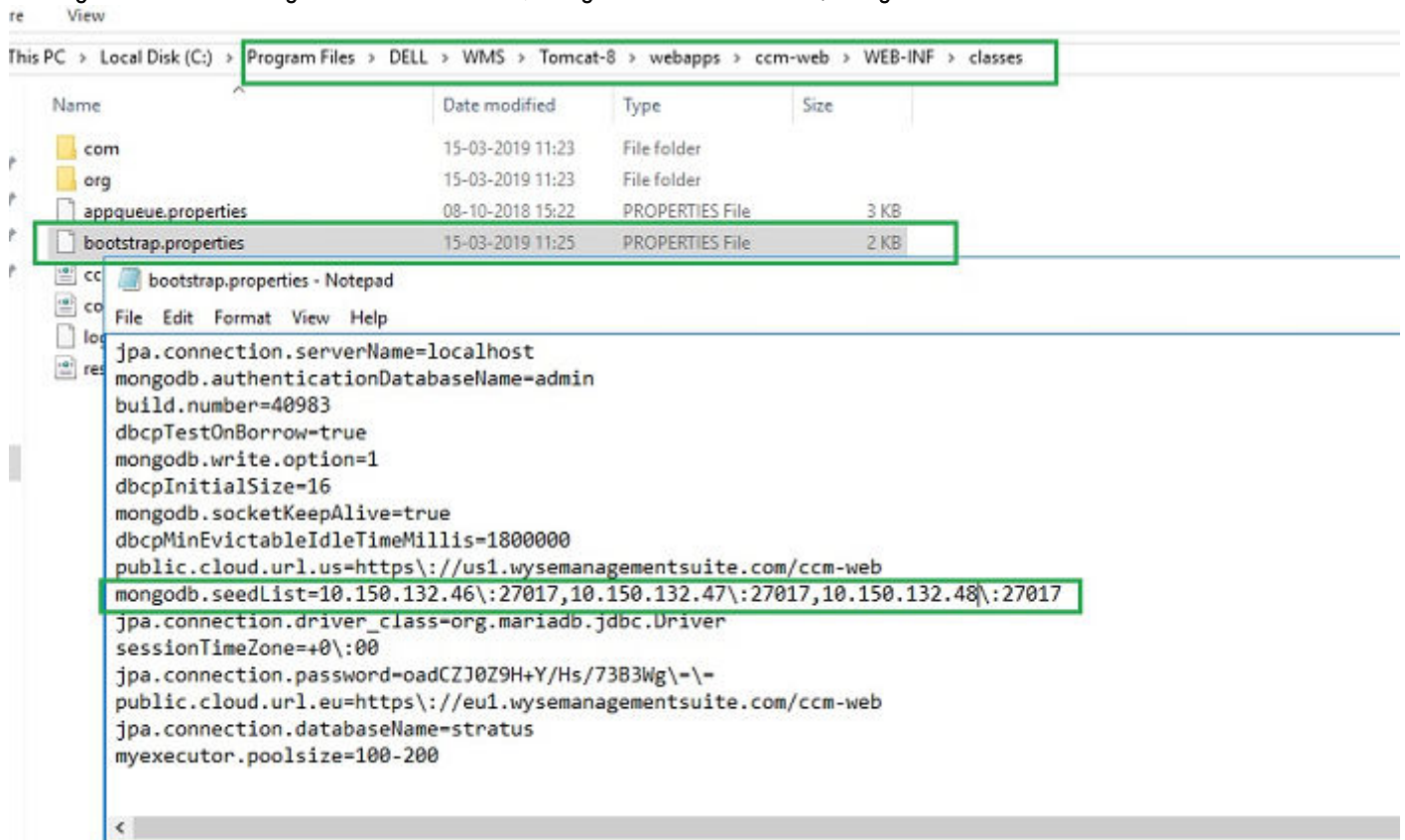
Figure 62. Prerequisite
