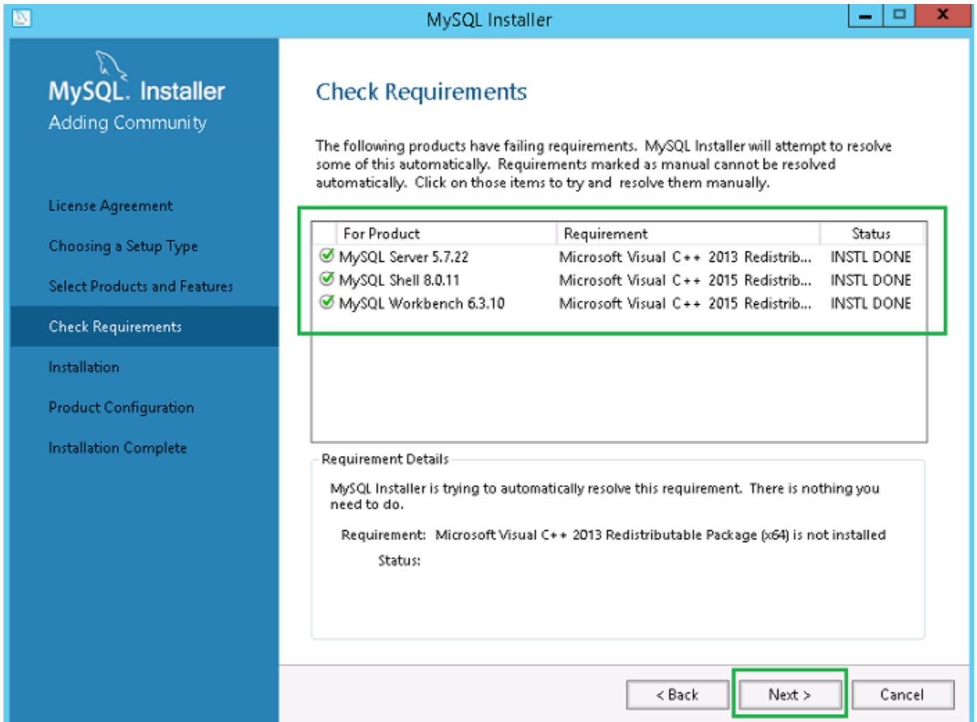
Figure 23. Configuration requise
