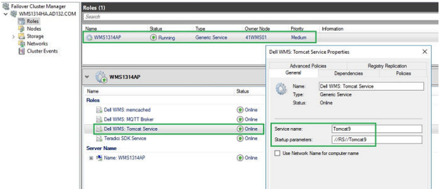
Figure 70. Service Tomcat 9
