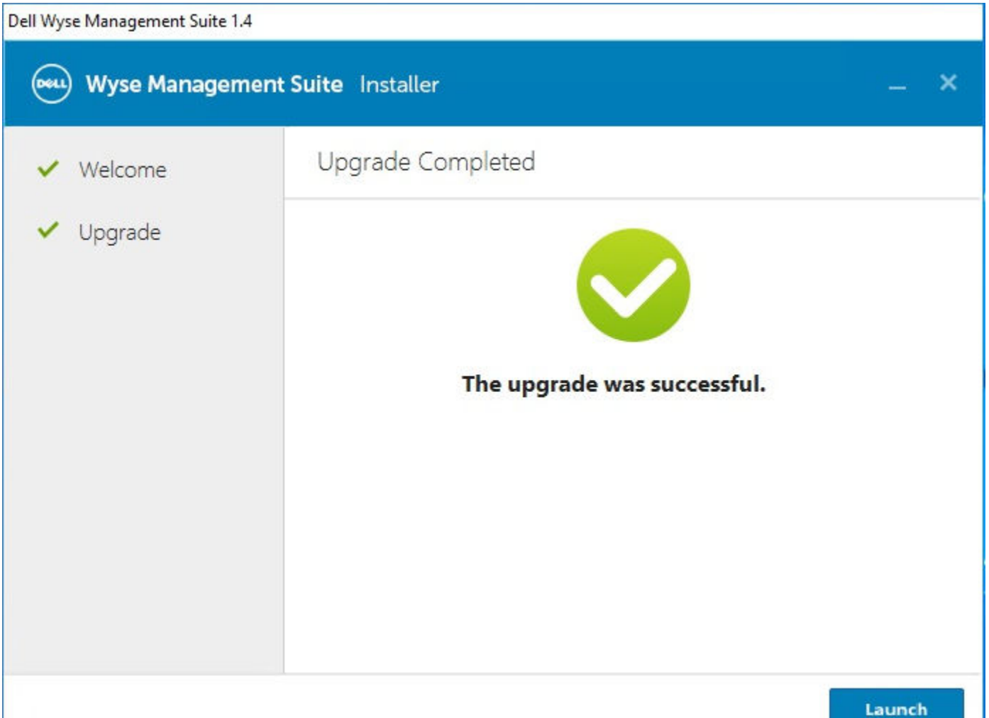
Figure 66. Lancer
