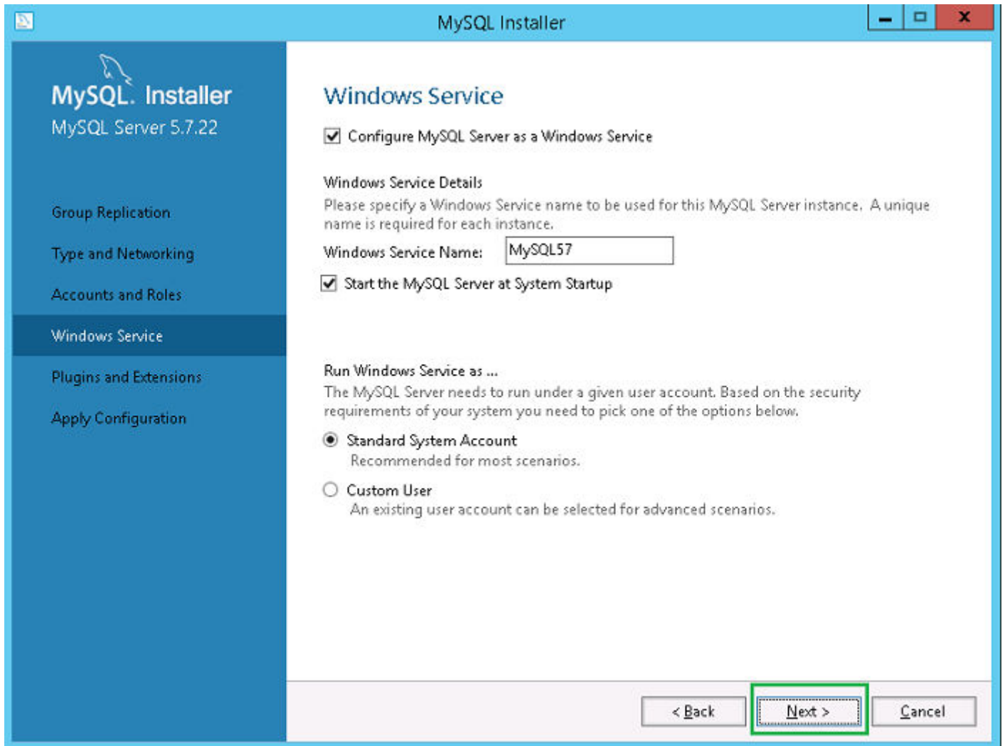
Figure 31. Service Windows
