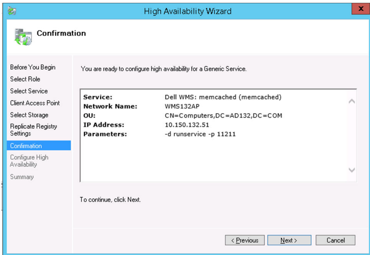
Figure 5. Confirmation
