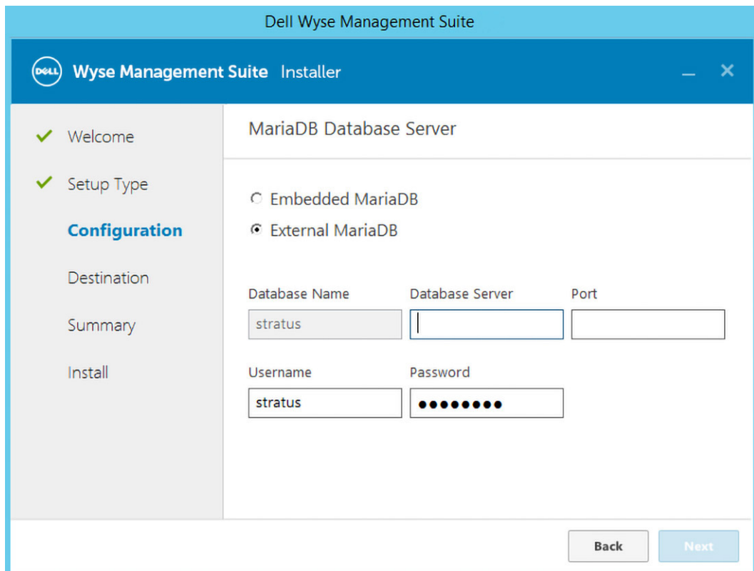
Figure 16. External MariaDB
