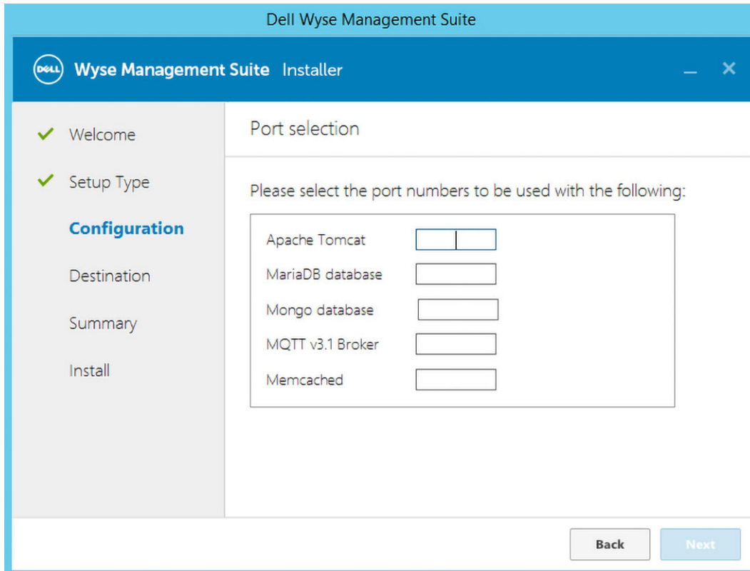
Figure 17. Port selection
