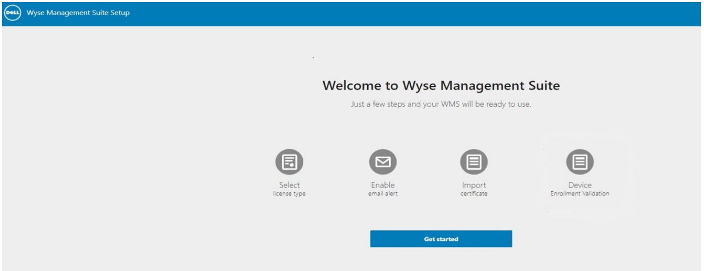
Figure 1. Welcome page
