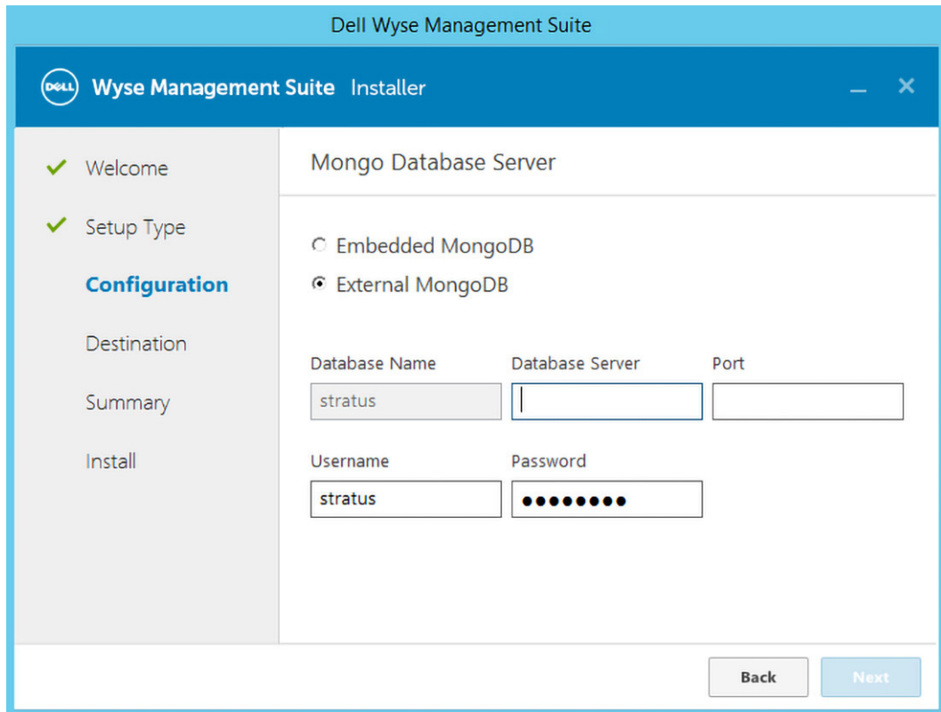
Figure 14. External MongoDB
