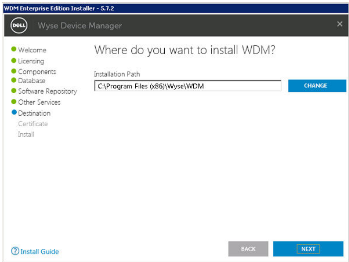
Figure 32. Destination Screen
