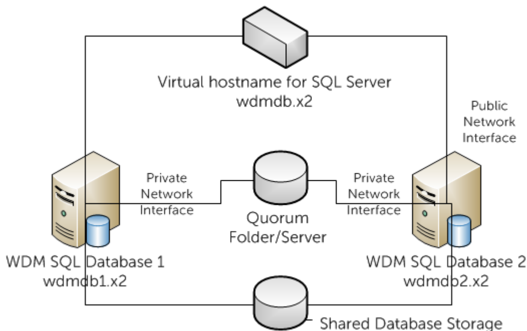
Figure 36. WDM High Availability Database Clustering
