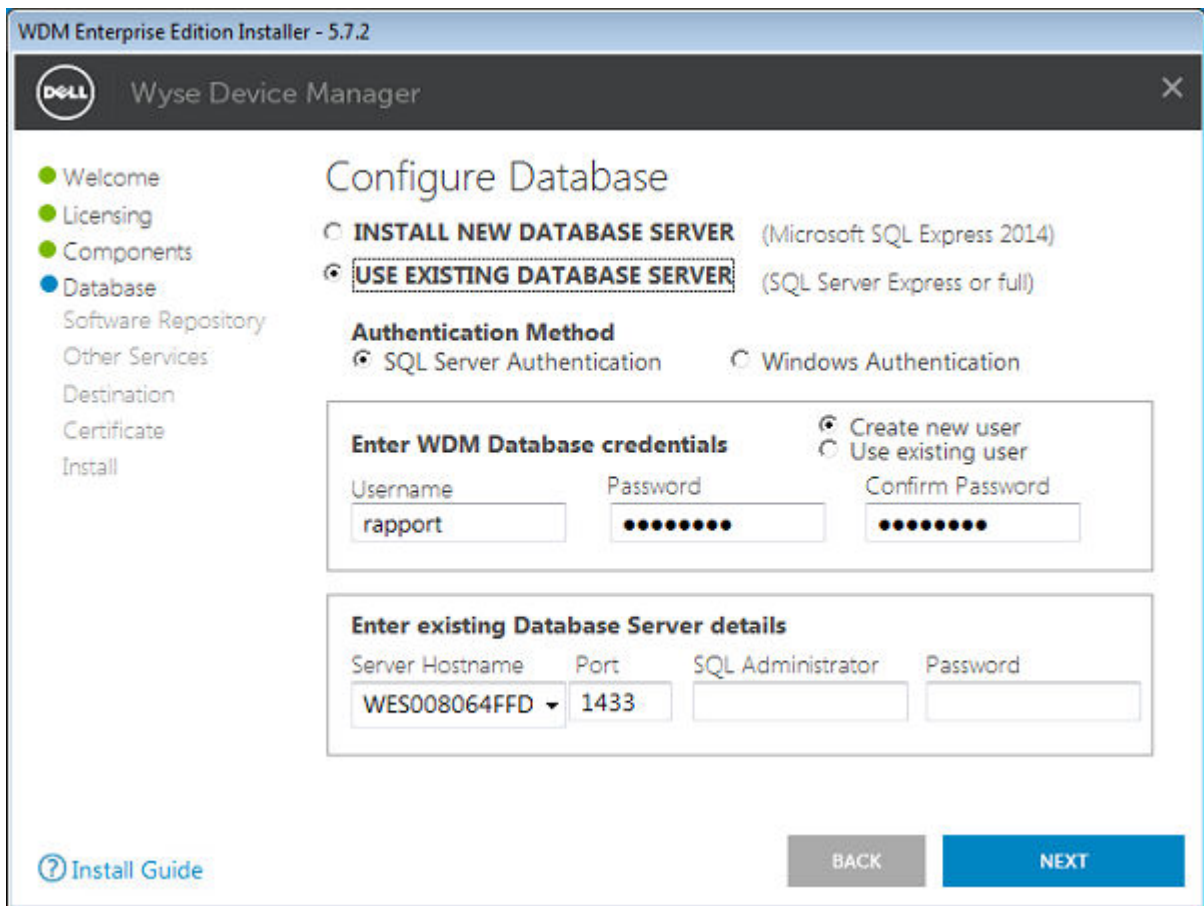
Figure 28. Existing Database Screen
