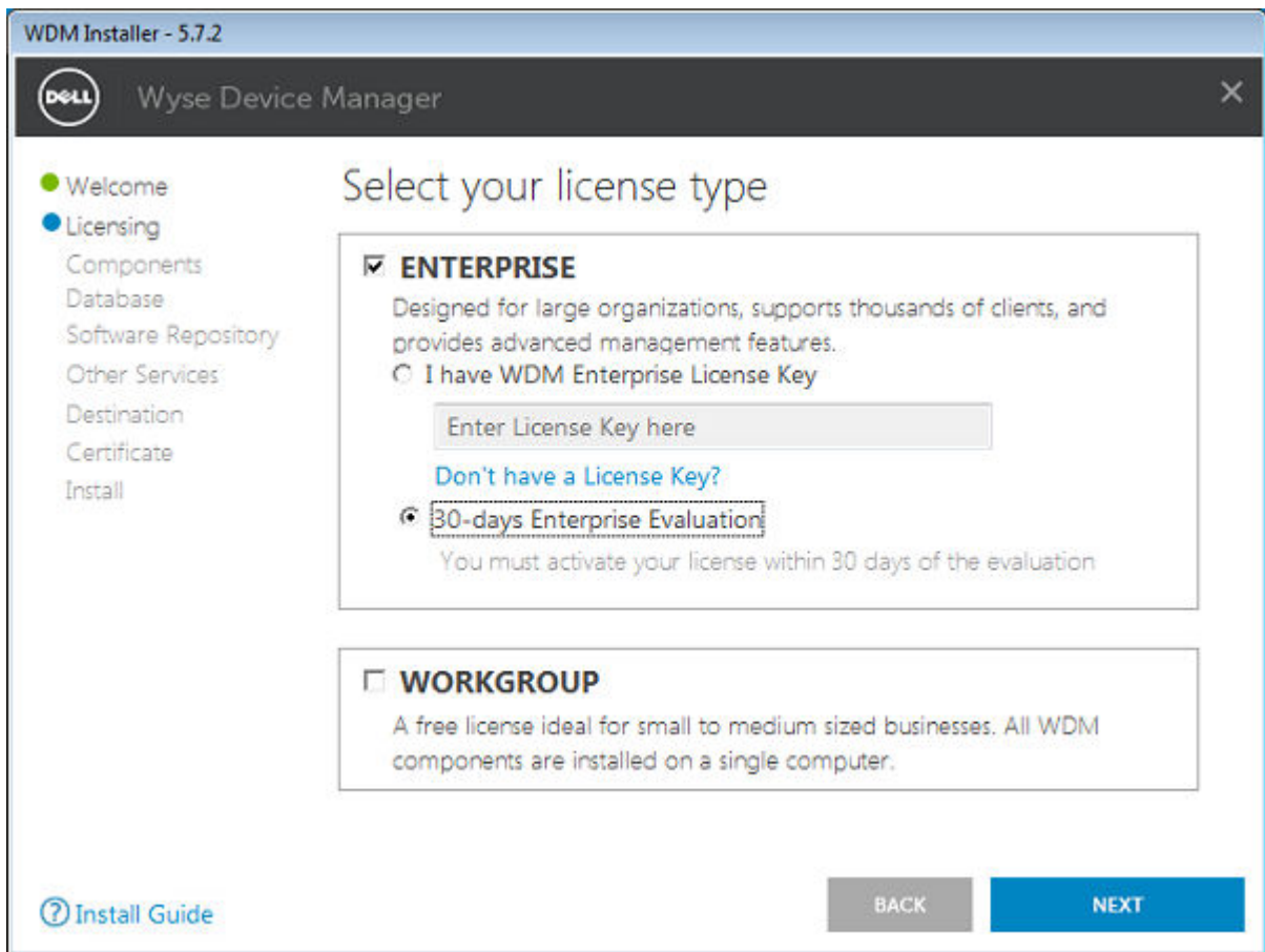
Figure 25. License Screen
