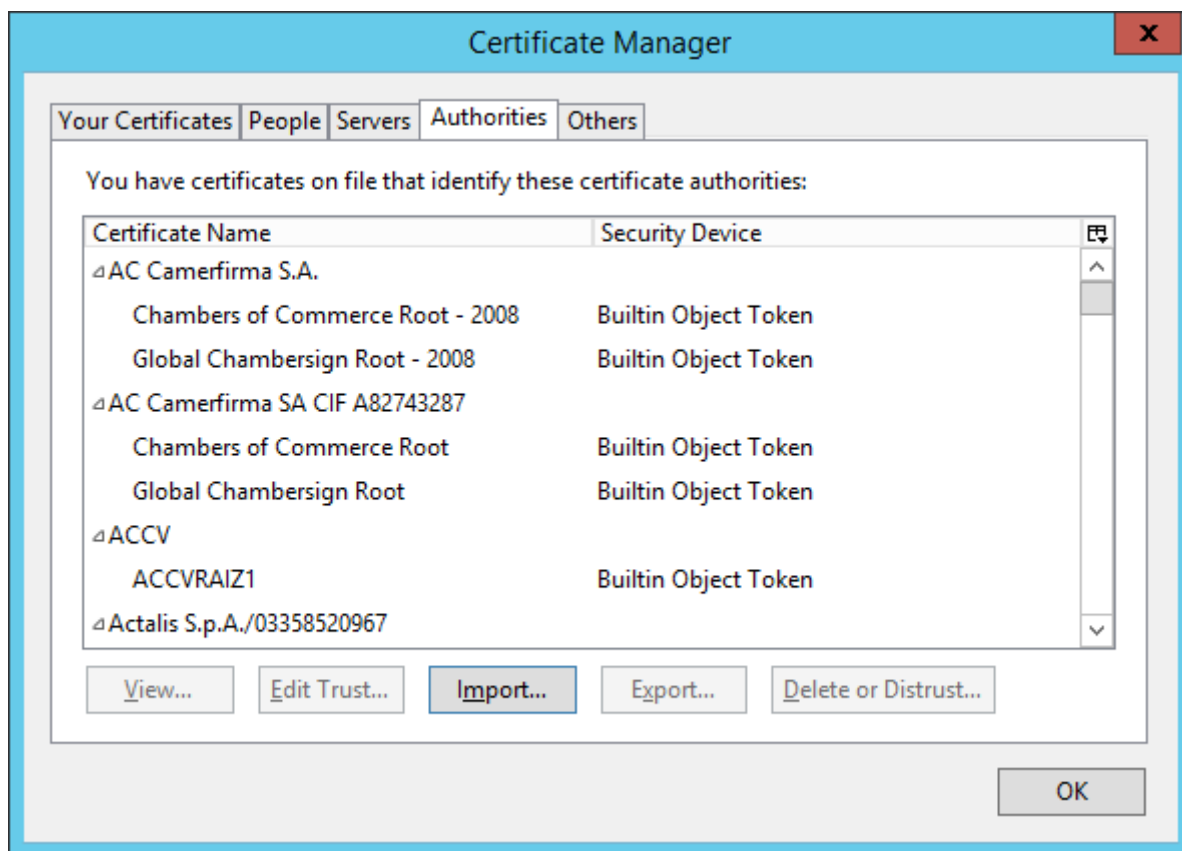
Figure 44. Certificate Manager
