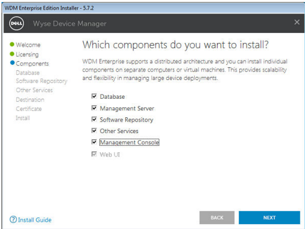
Figure 26. Components Screen
