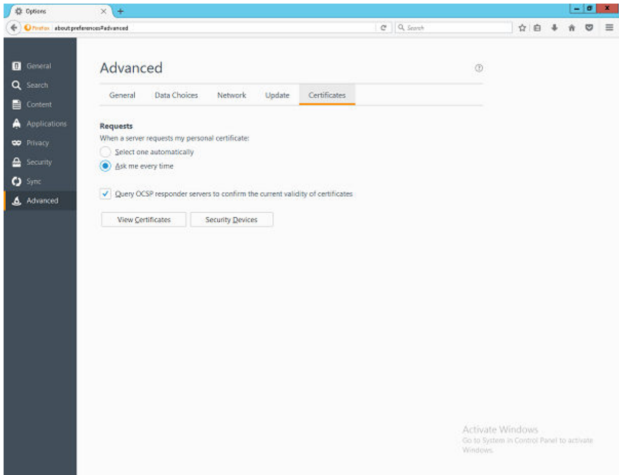
Figure 43. Advanced
