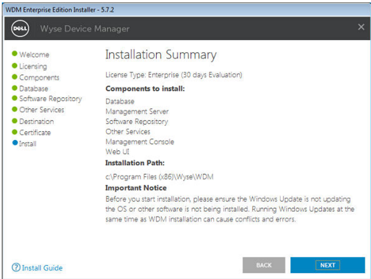
Figure 23. Installation Summary
