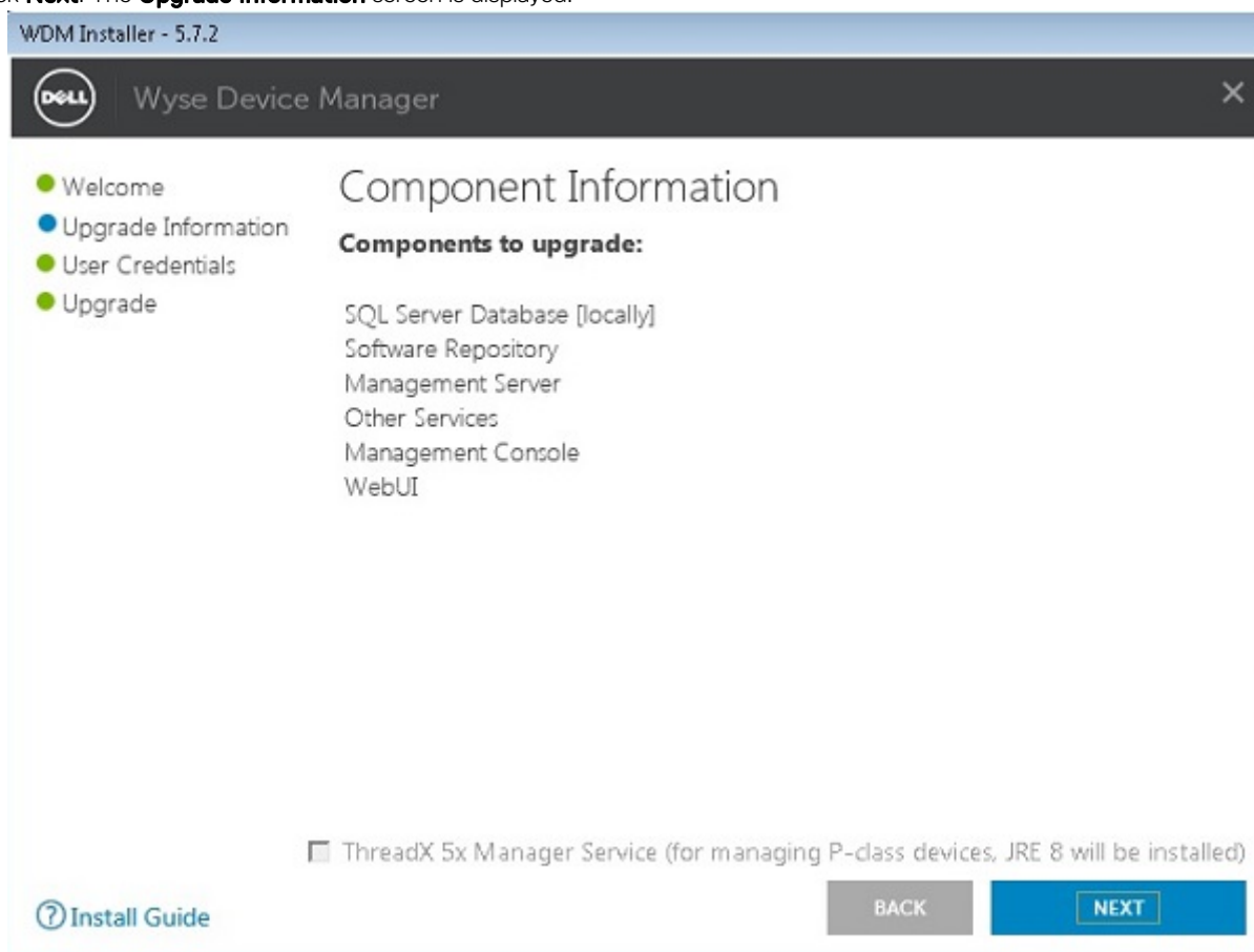
Figure 35. Component Information
