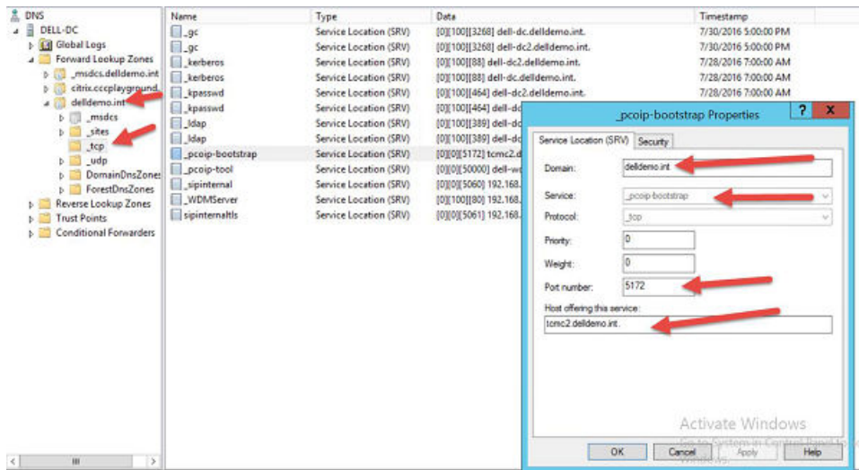
Figure 74. DNS_SRV record for _pcyip-bootstrap
