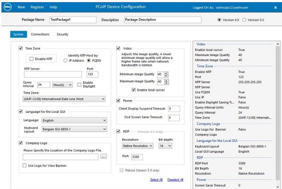
Figure 21. System Version 4.X
