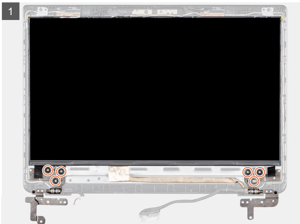
6x M2.5x3.5
