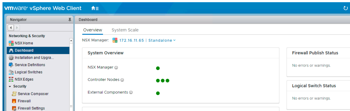
Figure 53. NSX dashboard
