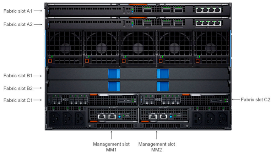
Figure 4. PowerEdge MX7000 chassis—rear view
