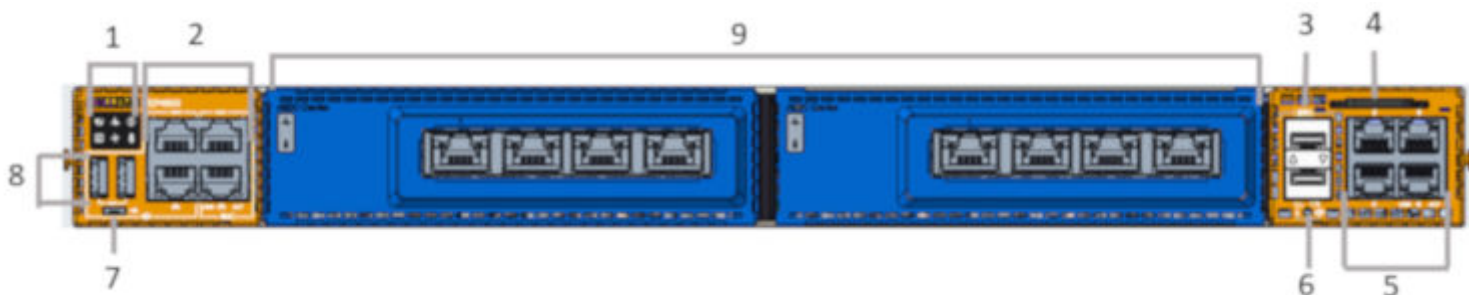
Figure 2. VEP4600 I/O-side view
