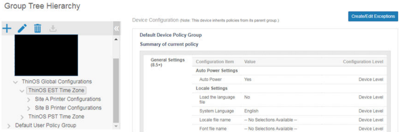
Figure 1. Device policy
