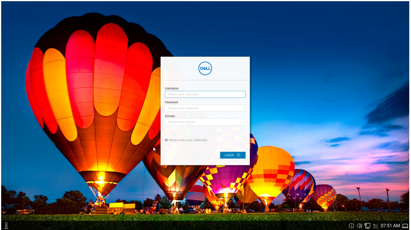
Figure 10. Classic desktop
