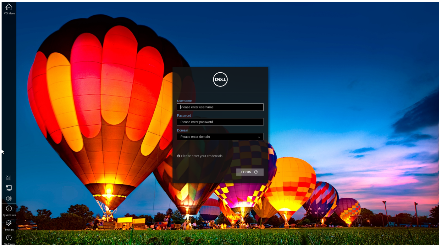
Figure 9. Modern desktop
