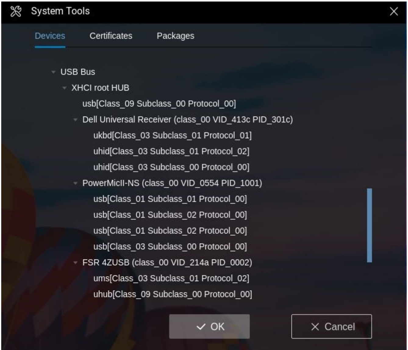
Figure 26. USB redirection
