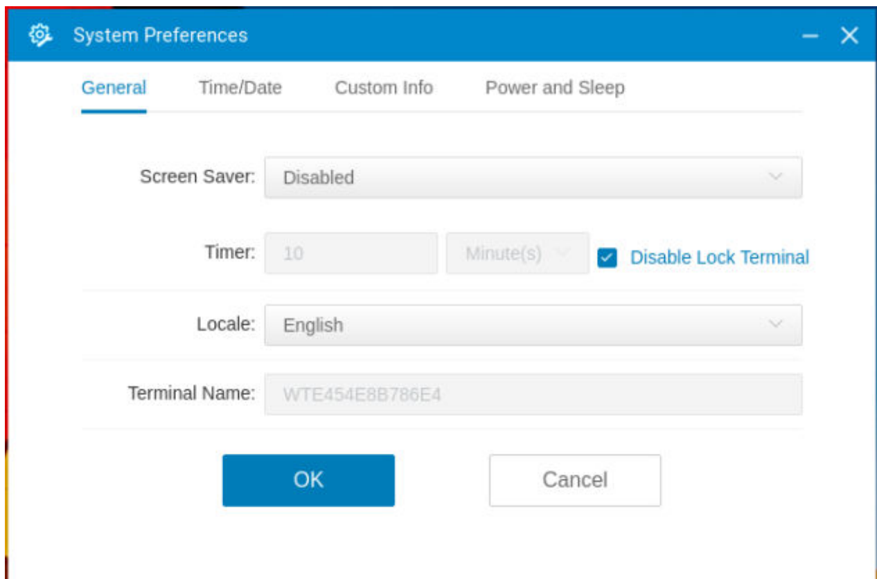
Figure 37. General tab
