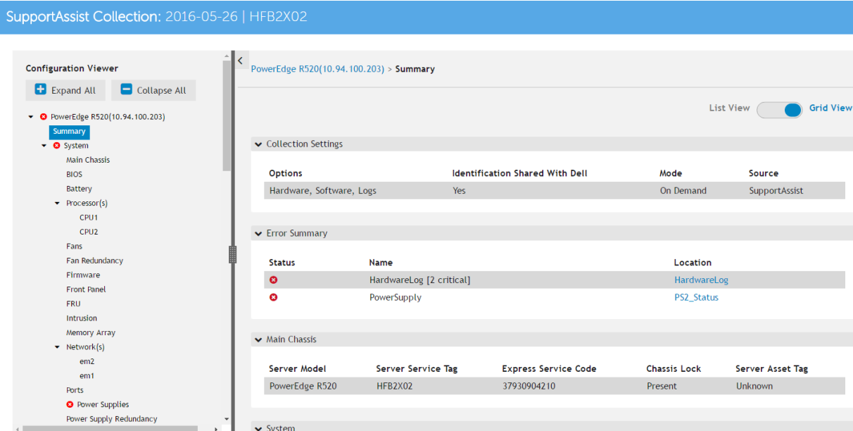
Figure 40. Configuration Viewer
