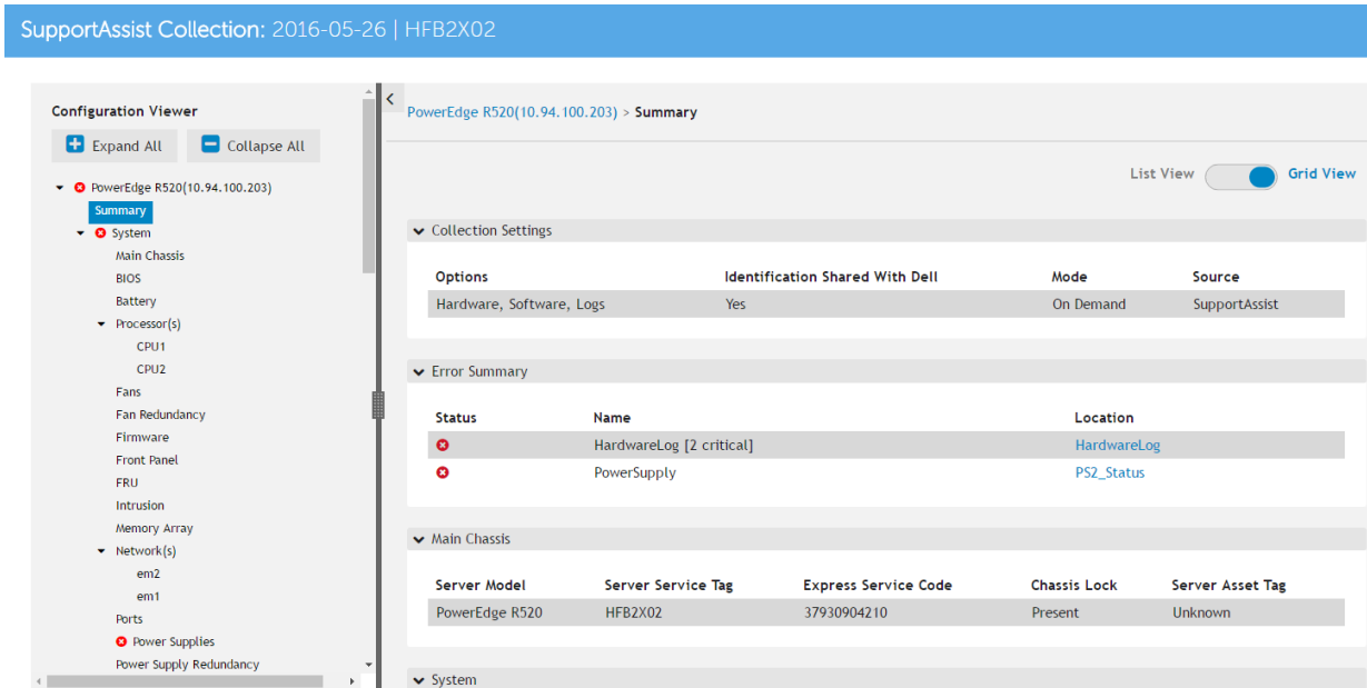
Figure 42. Configuration Viewer
