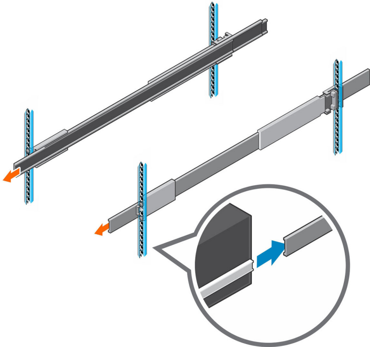
Figure 7. Extend the Rack Rails
