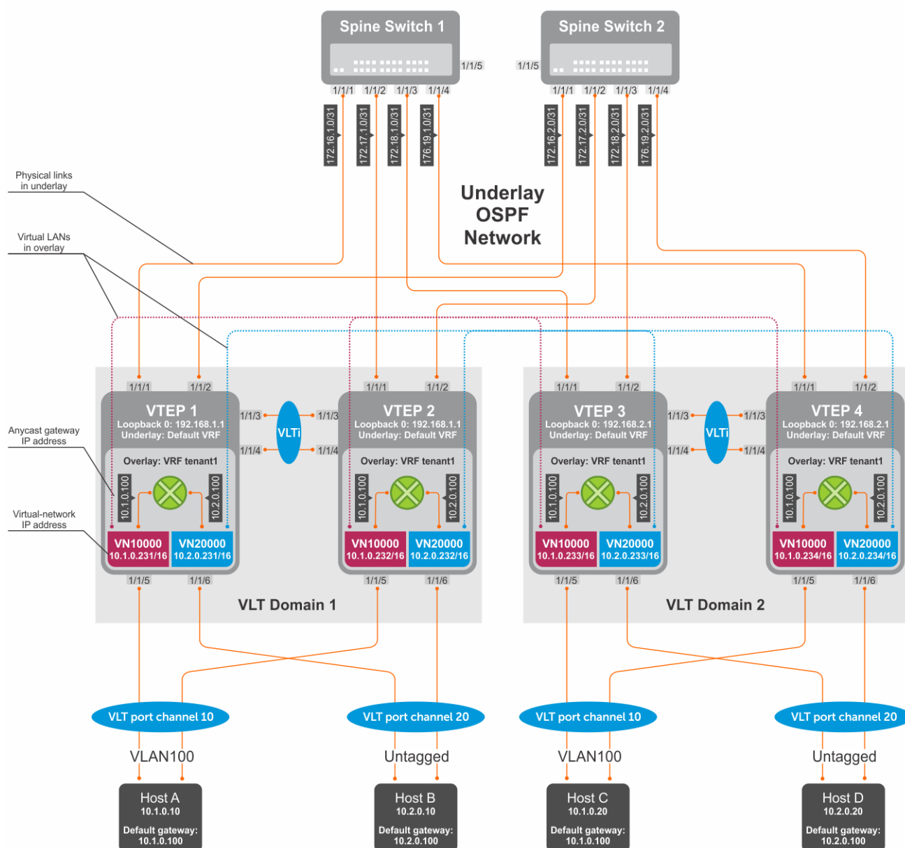
Figure 10. Static VXLAN use case
