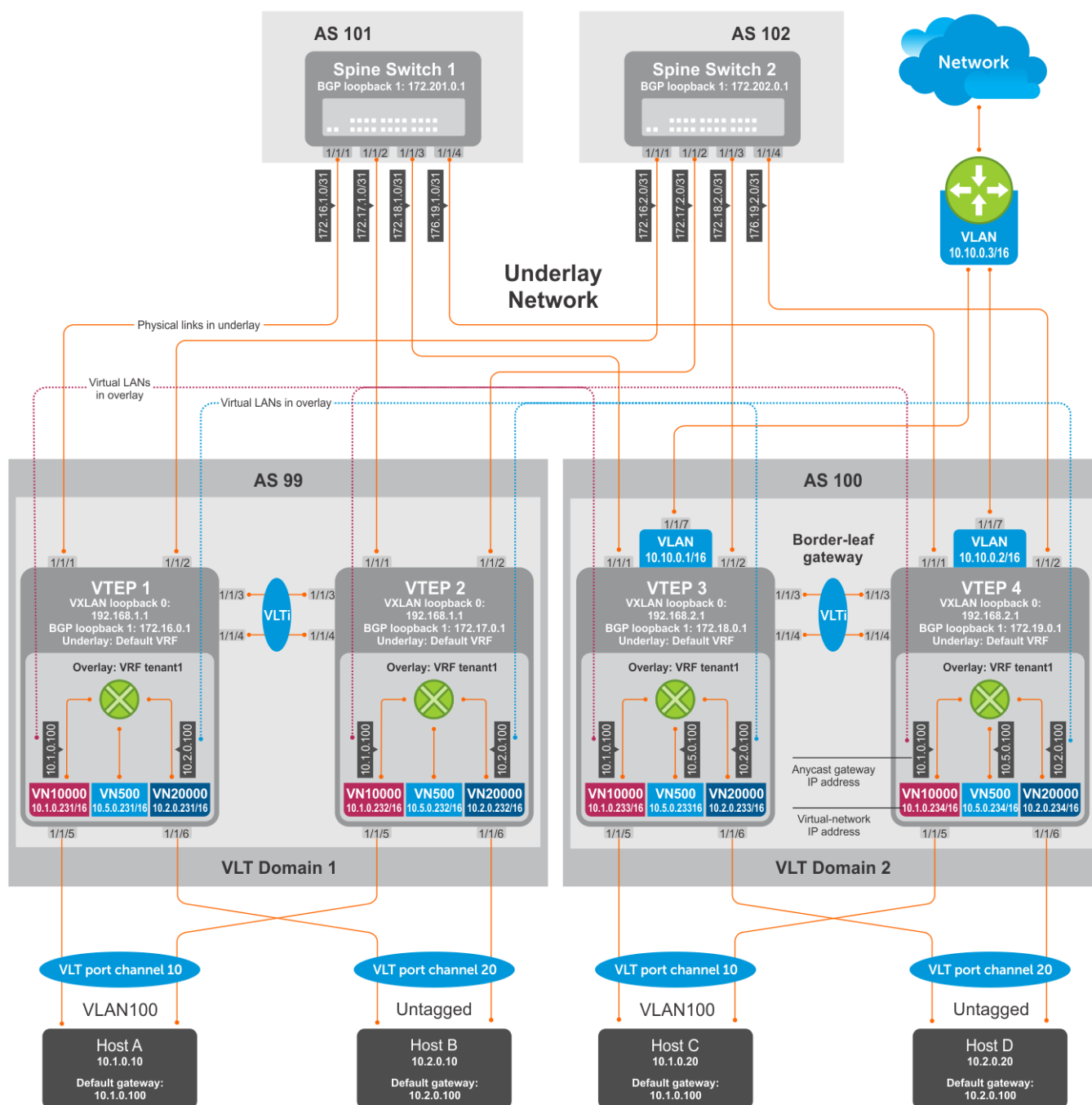
Figure 16. VXLAN BGP EVPN with border leaf gateway
