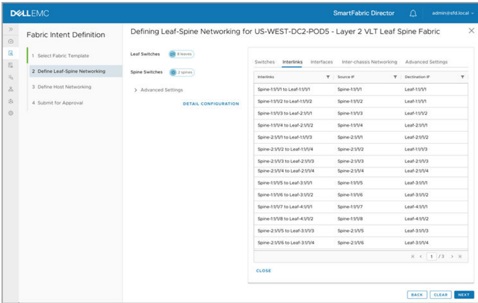
Details of interchassis configuration for Layer 2 fabric.
