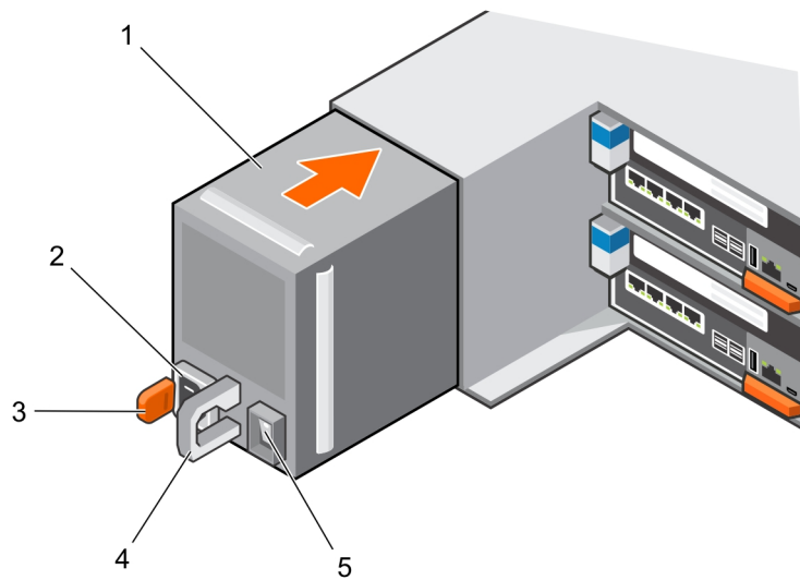
Figure 9. Removing a Power Supply/Cooling Fan Module
