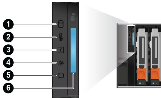
Figure 12. NVMe expansion enclosure front view status LEDs
