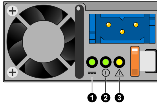
Figure 10. Base enclosure DC power supply LEDs
