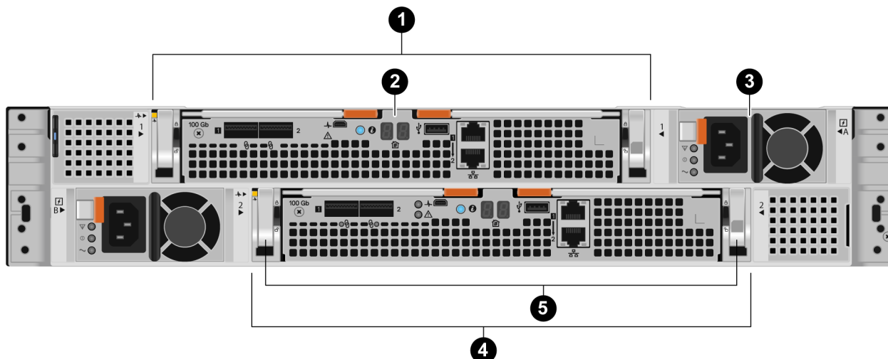
Figure 13. NVMe expansion enclosure rear component locations
