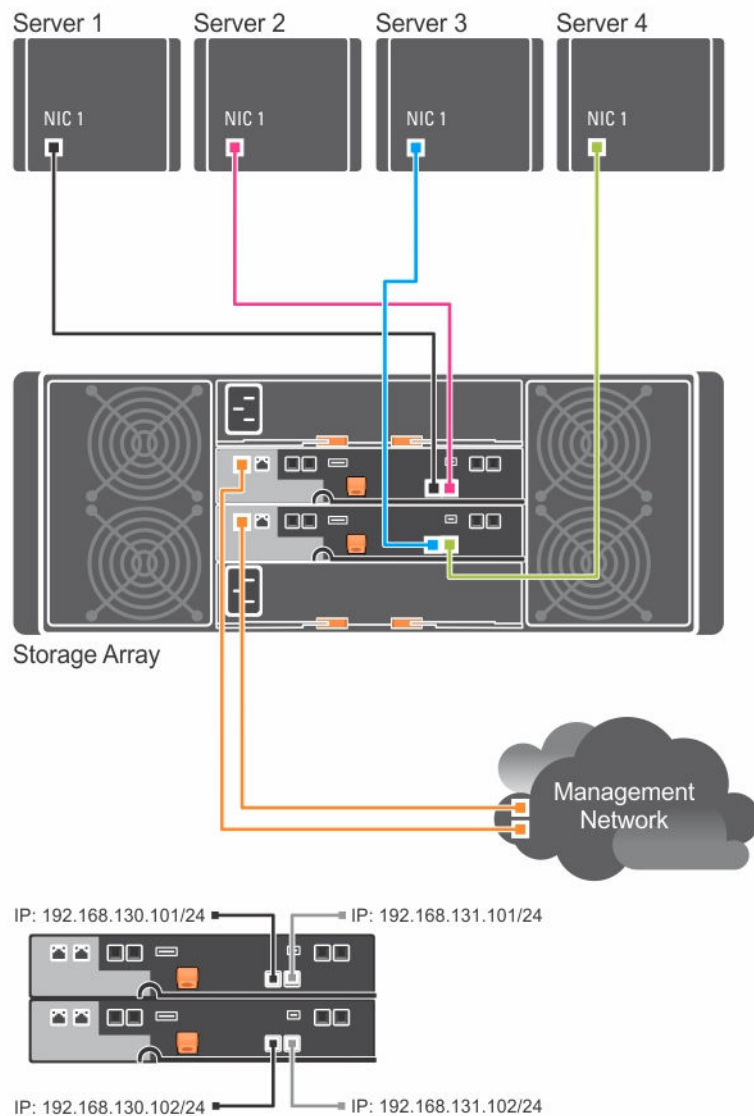
Figure 1. Four Hosts in a Dual-RAID Controller Configuration
