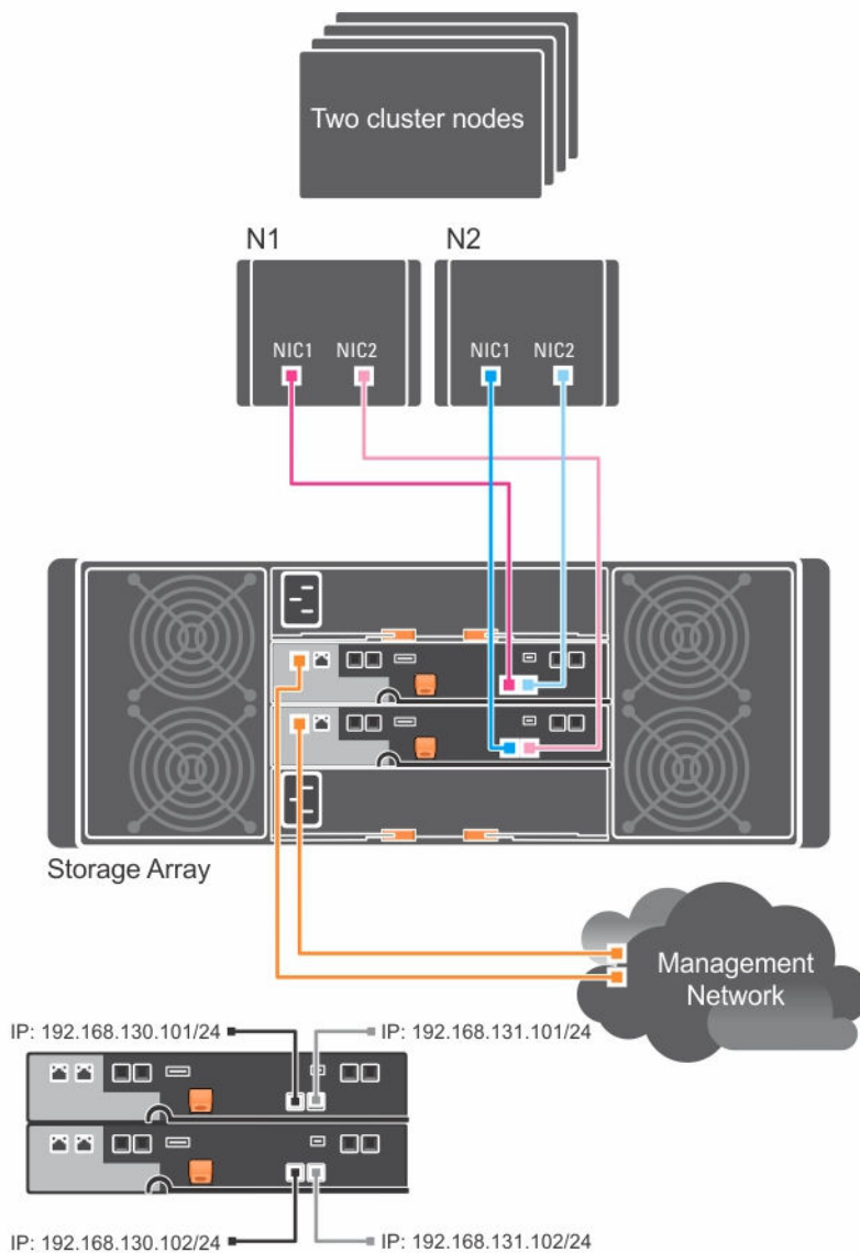
Figure 3. Two Cluster Nodes Connected to Two RAID Controllers
