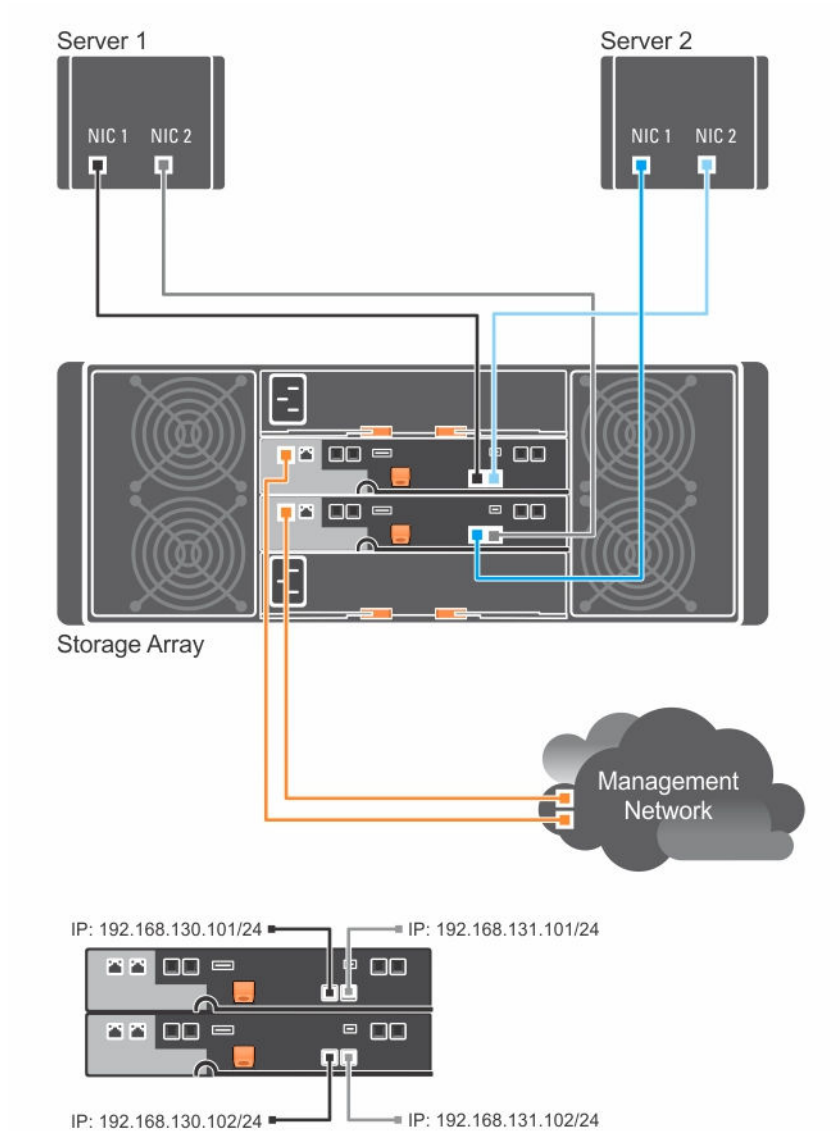
Figure 2. Two Hosts Connected to Two RAID Controllers
