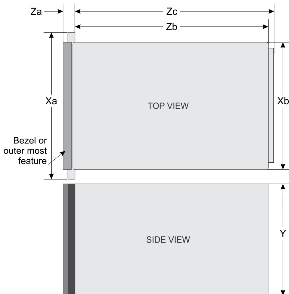
图 5: PowerEdge XE7100 机柜的尺寸
