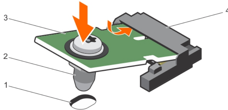
Figure 93. Installation du module TPM
