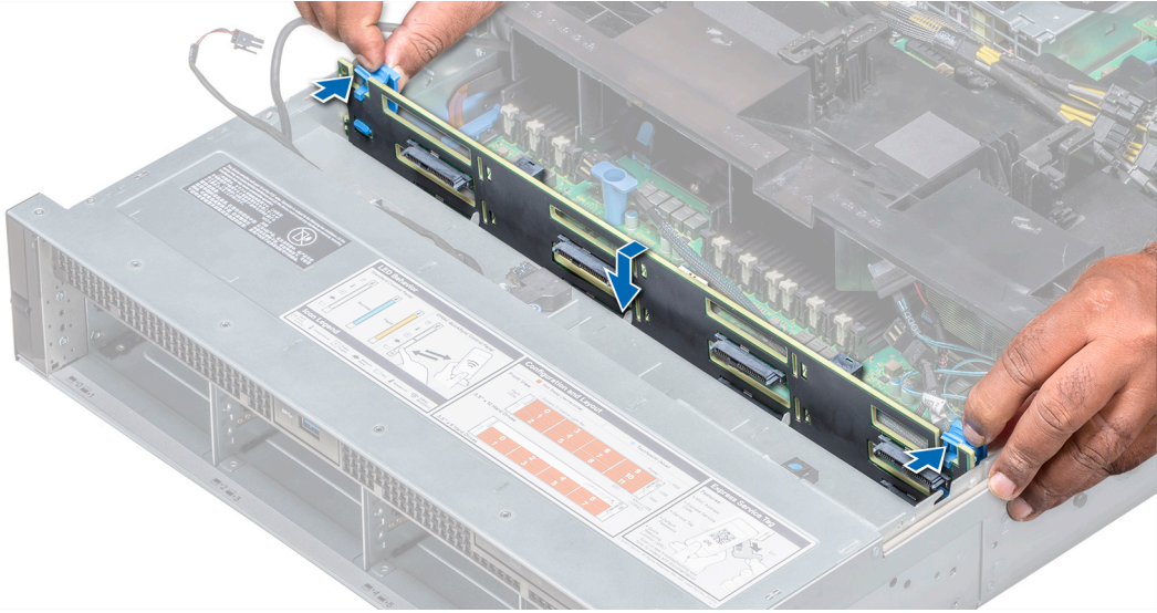
Rakam 132. Arka paneli takma
