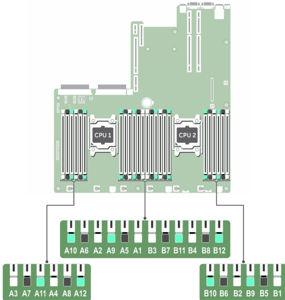
Figure 35. Emplacement des supports de mémoire
