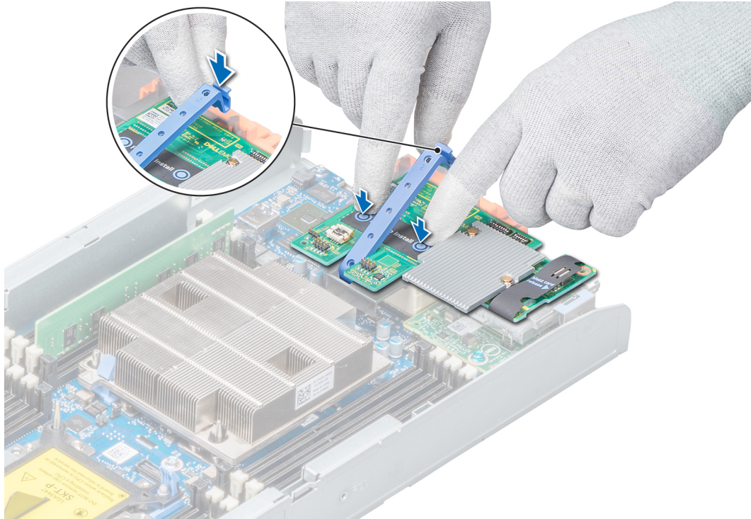
Figure 41. Installation de la carte mezzanine PCIe
