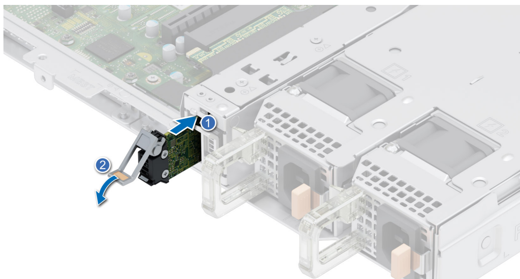
Figure 58. Installation du support de la carte BOSS S2
