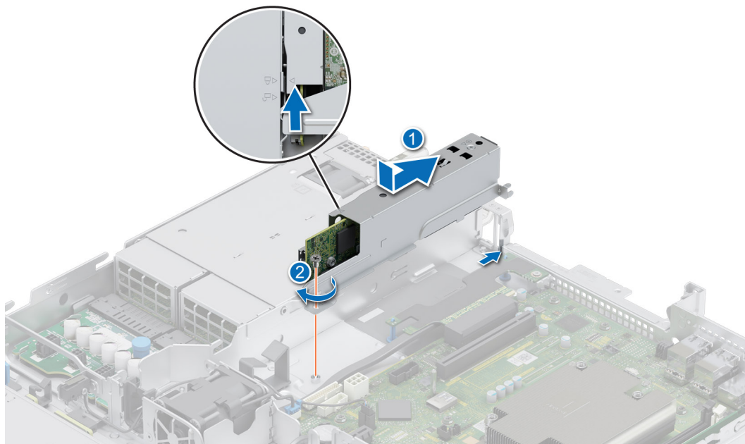
Figure 57. Installation du module BOSS S2
