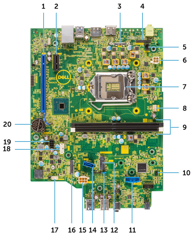
Small form factor board components (Liten formfaktor for moderkortoppsett)
