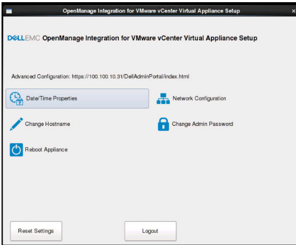
Figure 1. Onglet Console
