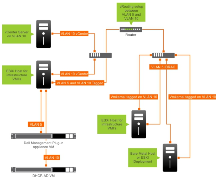
Figure 2. VLAN network.
