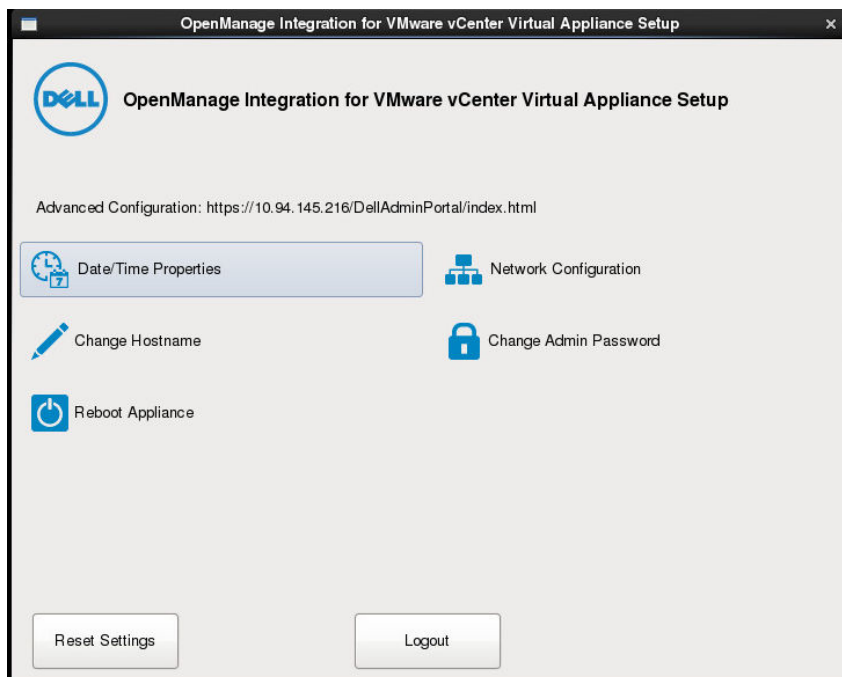
Figure 1. Onglet Console
