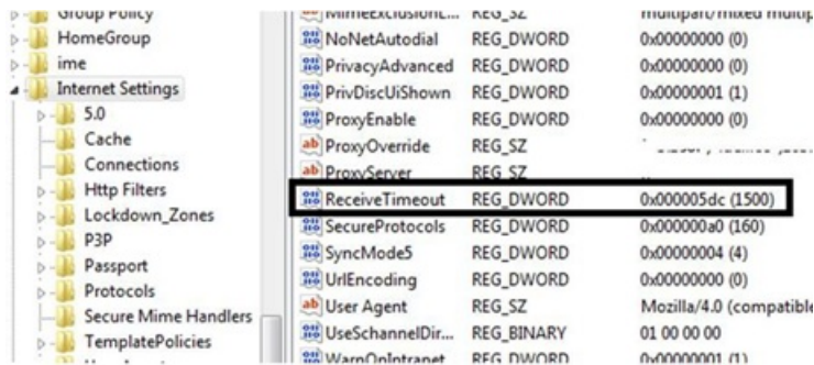
Figure 2. Registry
