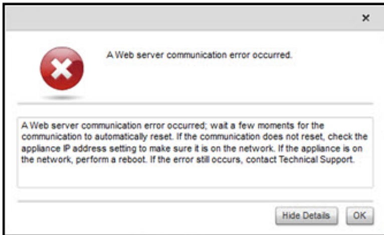
Figure 1. Communication error
