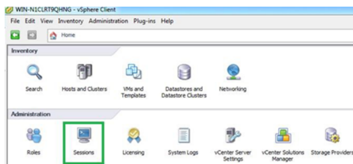
Figure 3. vSphere client
