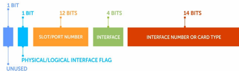
Figure 123. Example of Assigning Interface Index Numbers
