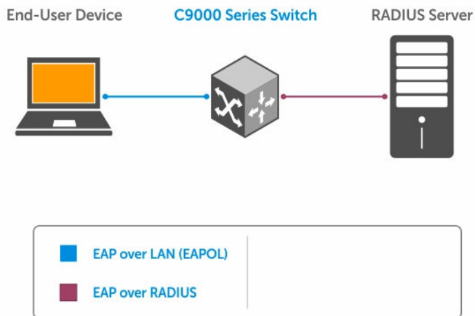
Figure 8. Single-Host Authentication Mode
