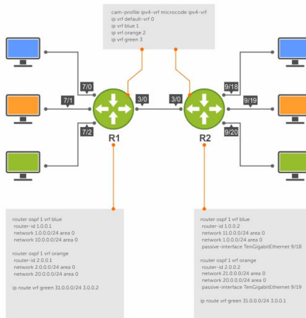
Figure 137. Setup OSPF and Static Routes
