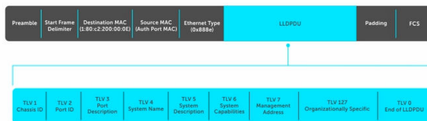
Figure 74. LLDPDU Frame
