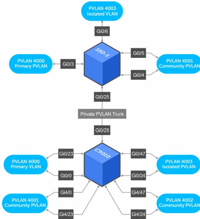
Figure 110. Sample Private VLAN Topology
