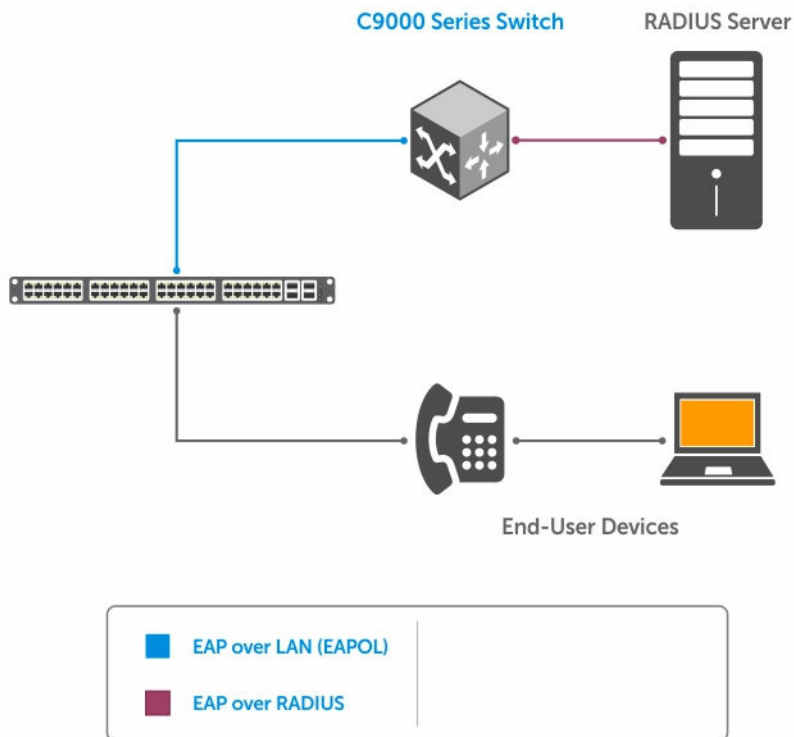
Figure 9. Multi-Host Authentication Mode
