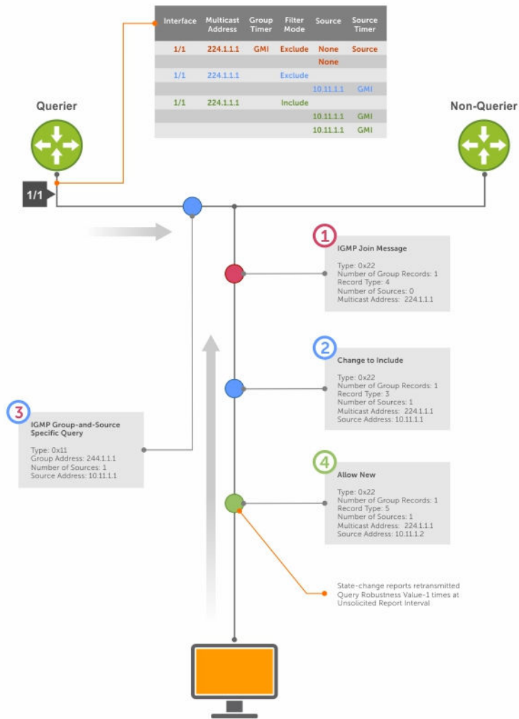
Figure 45. Membership Reports: Joining and Filtering
