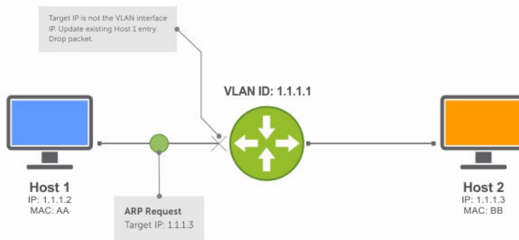
Figure 52. ARP Learning via ARP Request
