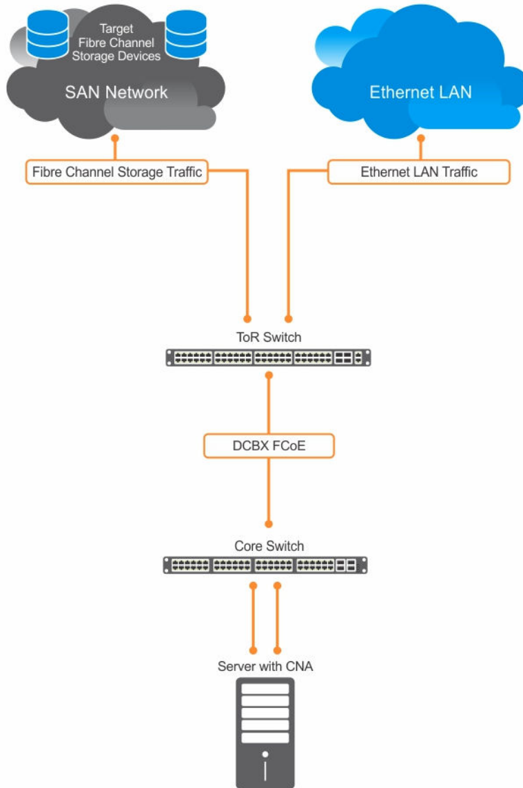
Figure 38. FIP Snooping on an Core Switch
