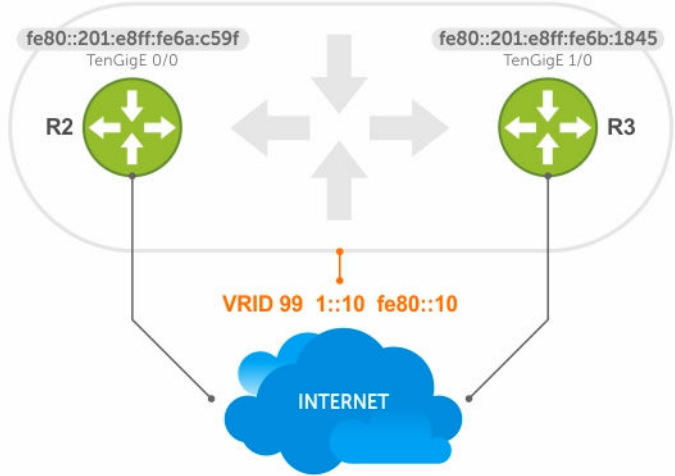
Figure 144. VRRP for an IPv6 Configuration
