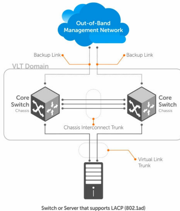
Figure 139. Example of VLT Deployment
