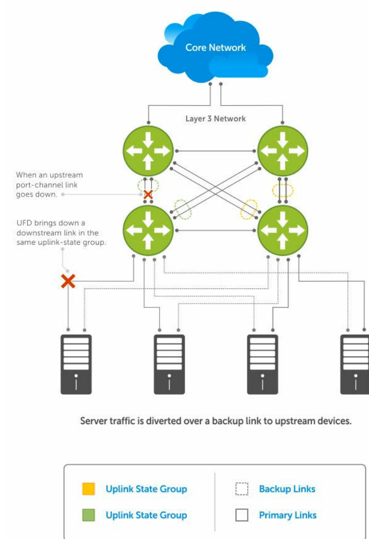
Figure 131. Uplink Failure Detection
