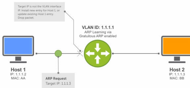
Figure 53. ARP Learning via ARP Request with ARP Learning via Gratuitous ARP Enabled
