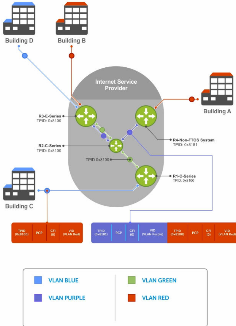
Figure 117. Single and Double-Tag TPID Match
