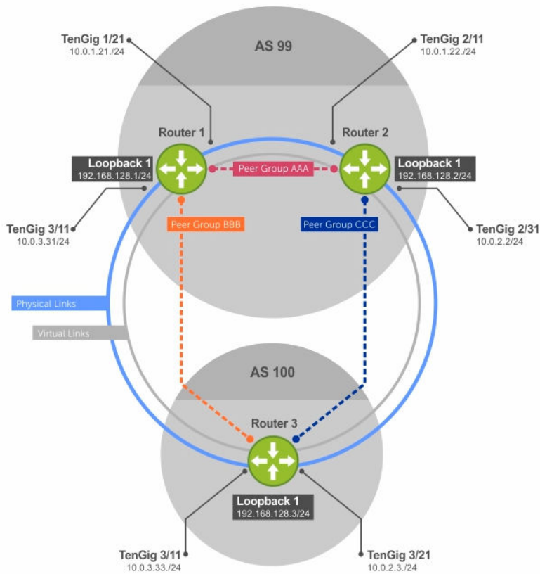
Figure 25. Sample Configurations
