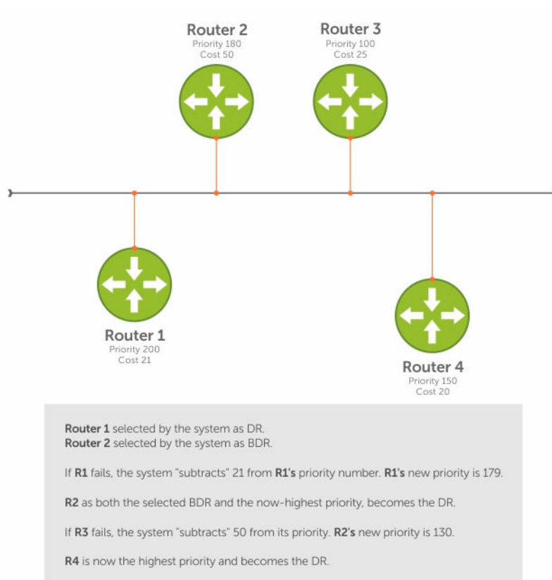
Figure 99. Priority and Cost Examples
