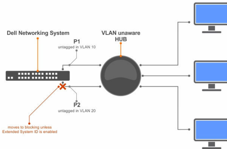
Figure 103. PVST+ with Extend System ID
