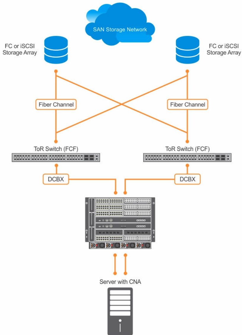
Figure 31. DCBx Sample Topology
