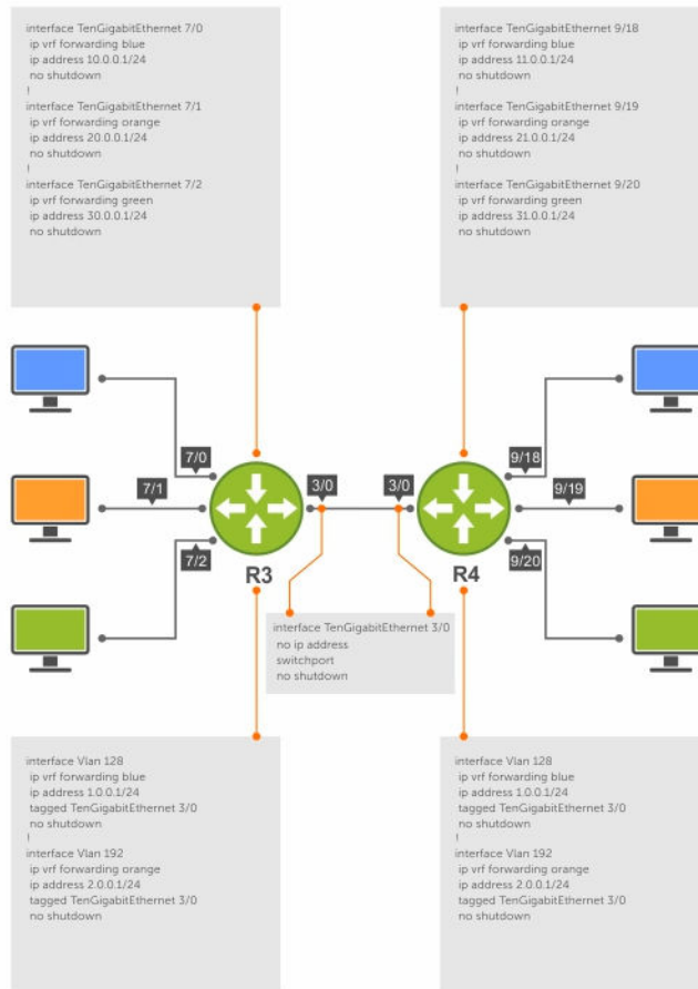
Figure 138. Setup VRF Interfaces
