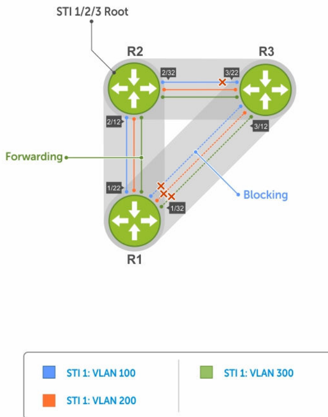
Figure 101. Per-VLAN Spanning Tree
