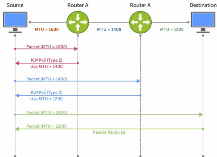
Figure 55. Path MTU Discovery Process
