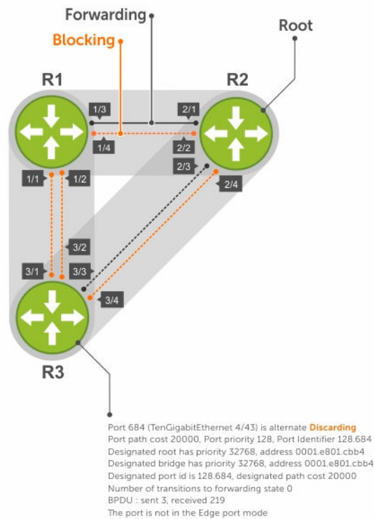
Figure 115. Rapid Spanning Tree Enabled Globally
