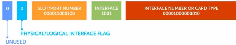
Figure 124. Interface Index Number Assigned to FortyGigE 0/4 Port
