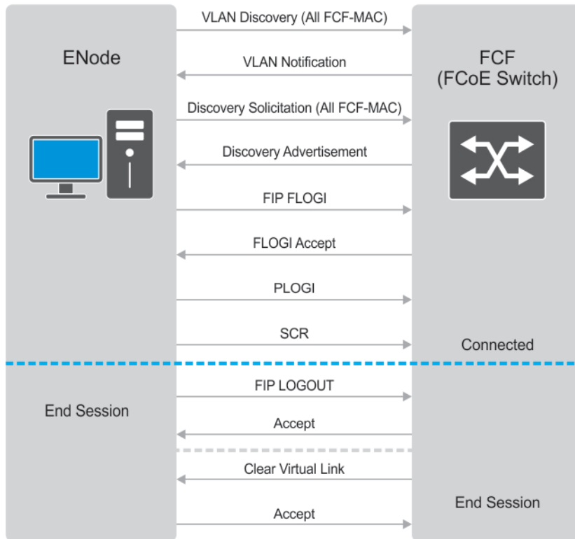
Figure 37. FIP Discovery and Login Between an ENode and an FCF
