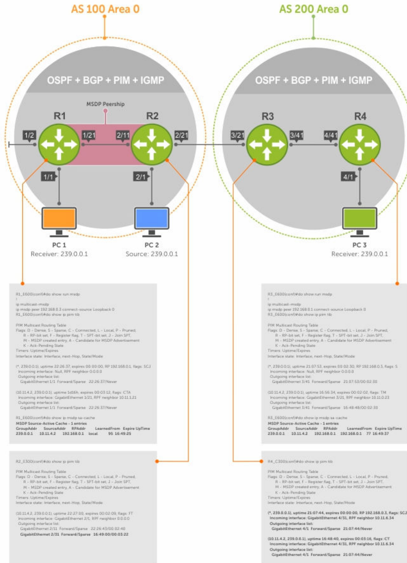
Figure 86. Configuring MSDP
