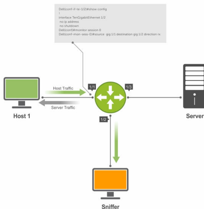
Figure 106. Port Monitoring Example
