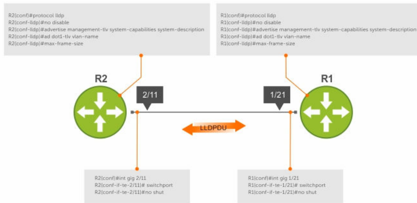
Figure 79. Configuring LLDP
