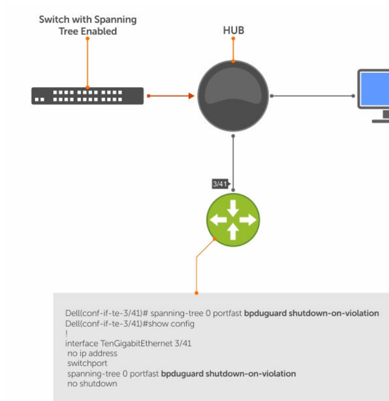
Figure 127. Enabling BPDUGuard
