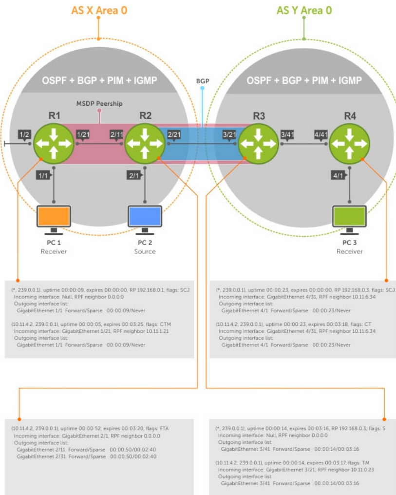
Figure 91. MSDP with Anycast RP
