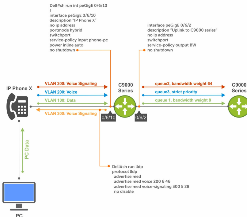
Figure 109. PoE VoIP Traffic
