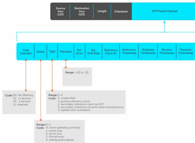
Figure 130. NTP Fields
