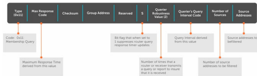
Figure 43. IGMP Version 3 Packet Structure
