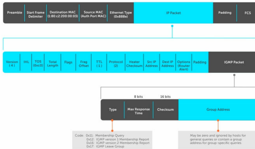
Figure 42. IGMP Messages in IP Packets
