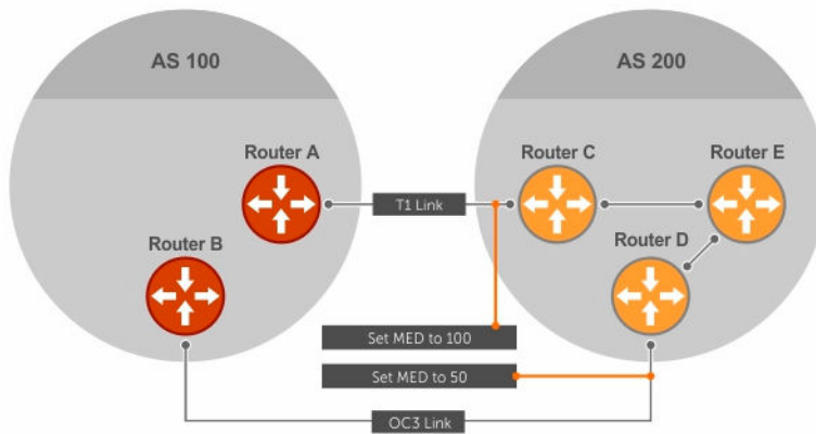
Figure 23. Multi-Exit Discriminators
