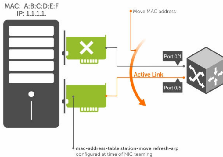
Figure 70. Configuring the mac-address-table station-move refresh-arp Command
