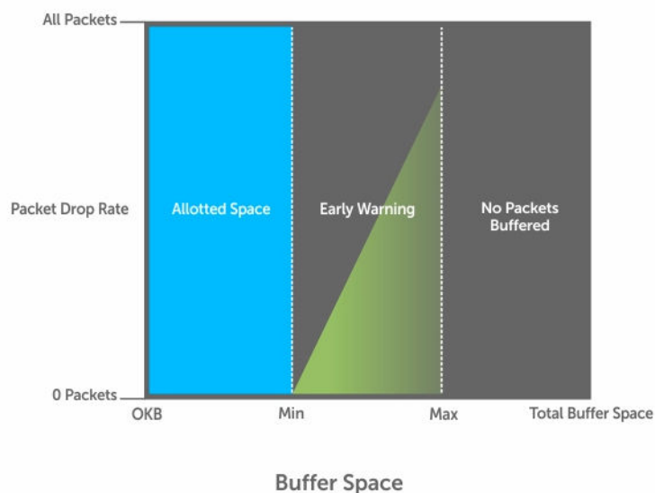
Figure 113. Packet Drop Rate for WRED
