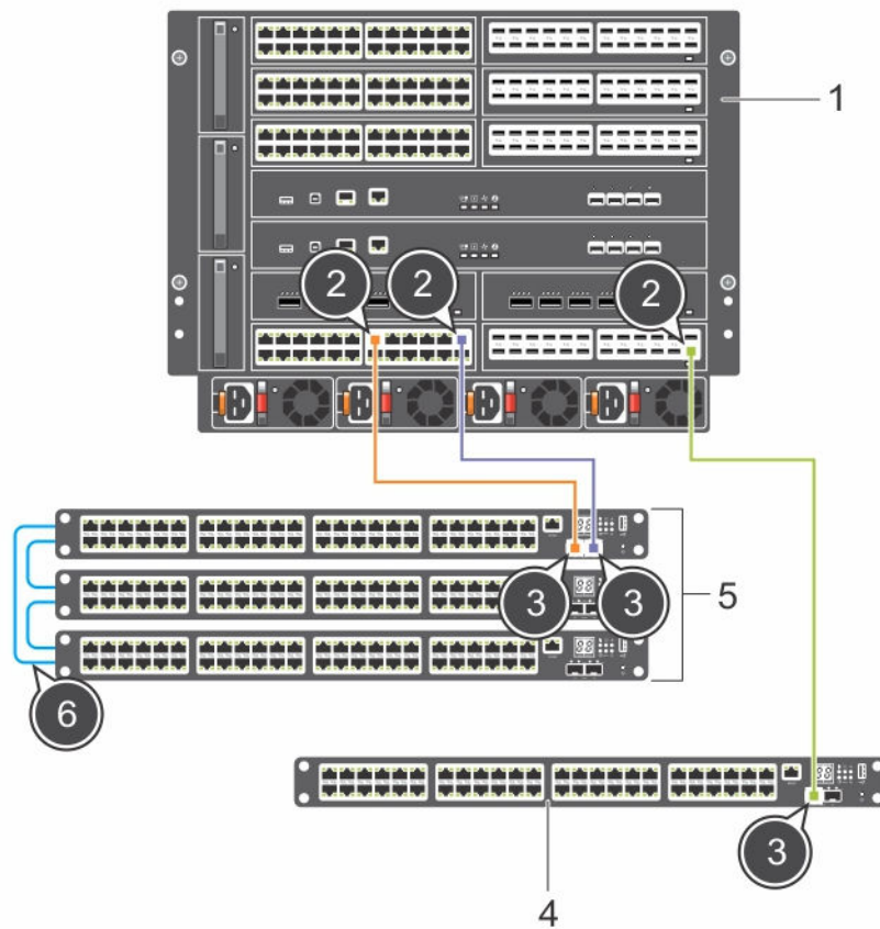
Figure 104. Controlling Bridge with Port Extenders
