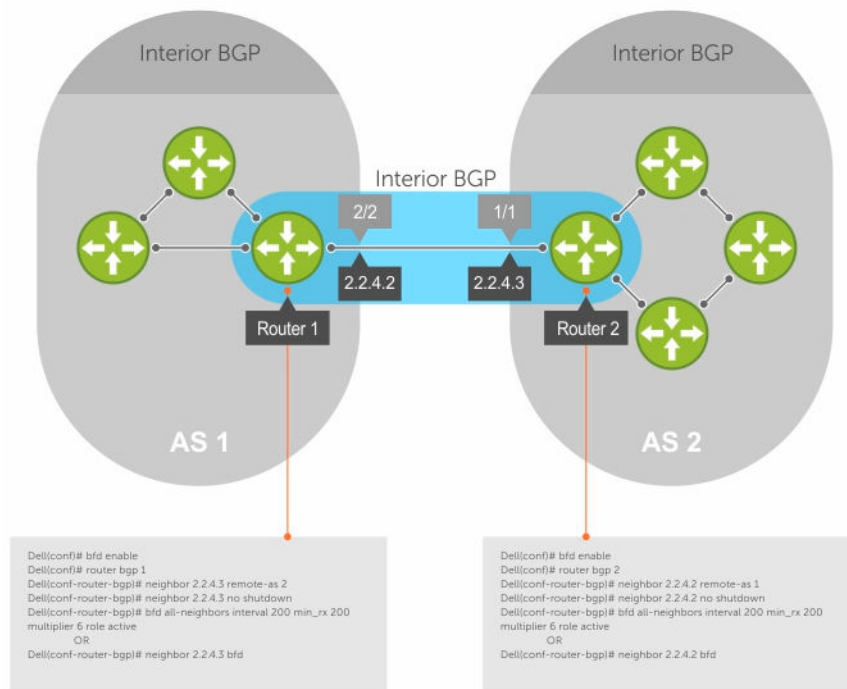
Figure 16. Establishing Sessions with BGP Neighbors
