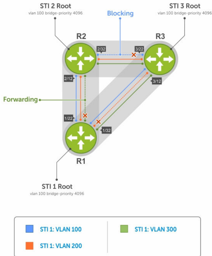
Figure 102. Load Balancing with PVST+
