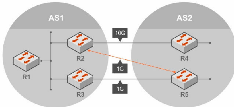
Figure 36. Sample BGP Link Bandwidth Configuration
