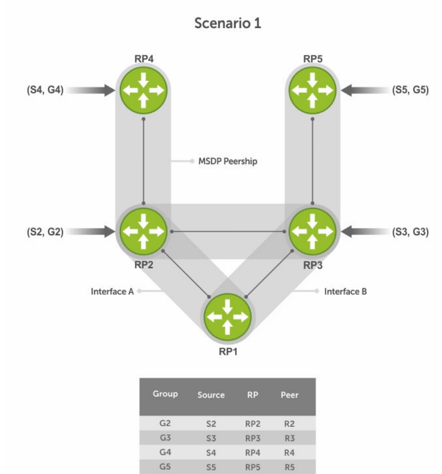
Figure 87. MSDP Default Peer, Scenario 1
