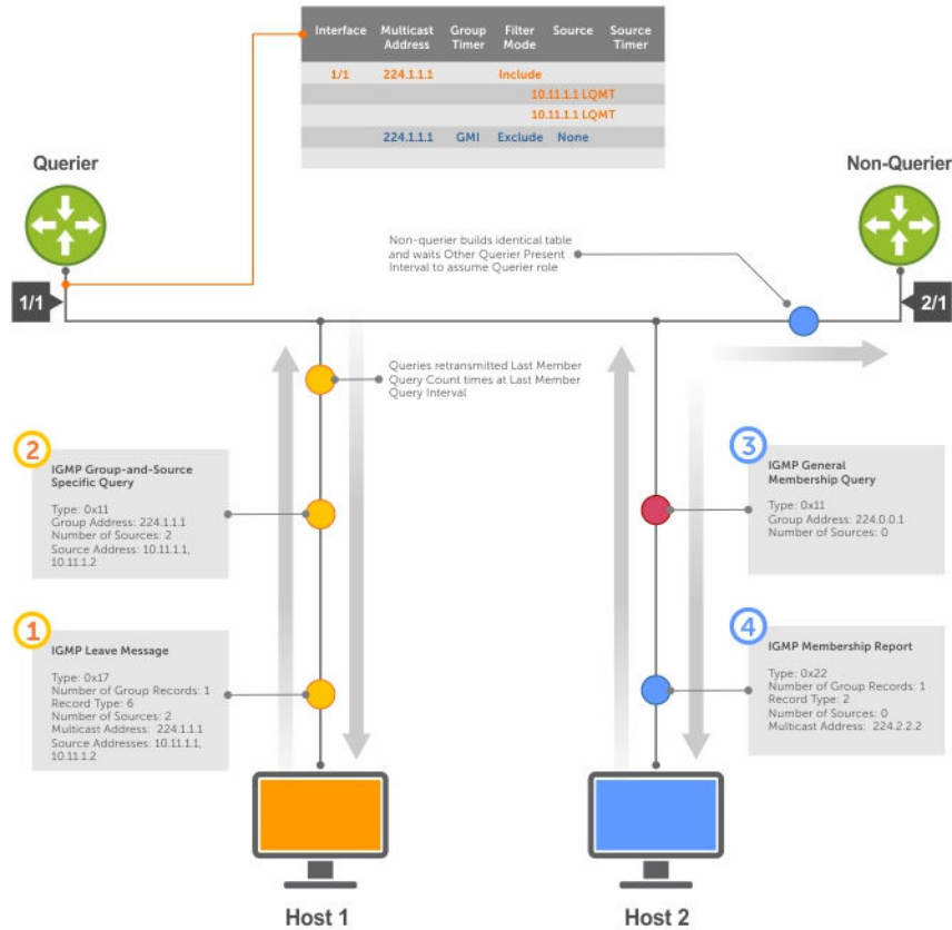
Figure 46. Membership Queries: Leaving and Staying
