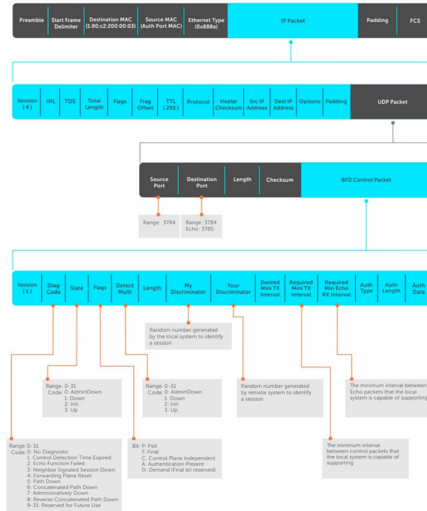
Figure 10. BFD in IPv4 Packet Format
