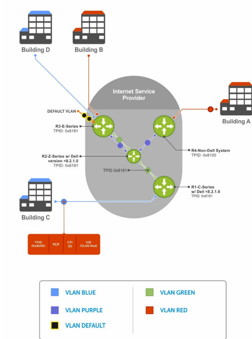
Figure 118. Single and Double-Tag First-byte TPID Match
