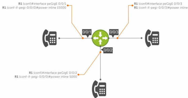
Figure 107. PoE Topology
