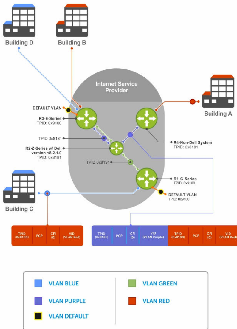
Figure 119. Single and Double-Tag TPID Mismatch
