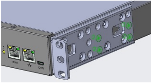
Five-inch-offset mount
