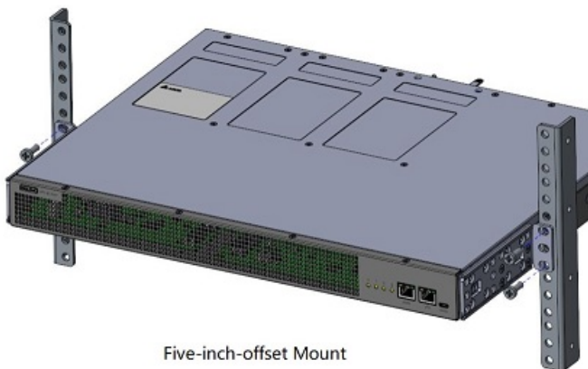
Five-inch-offset mount
