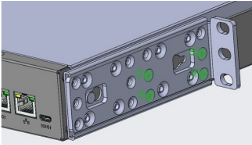
Five-inch-offset mount
