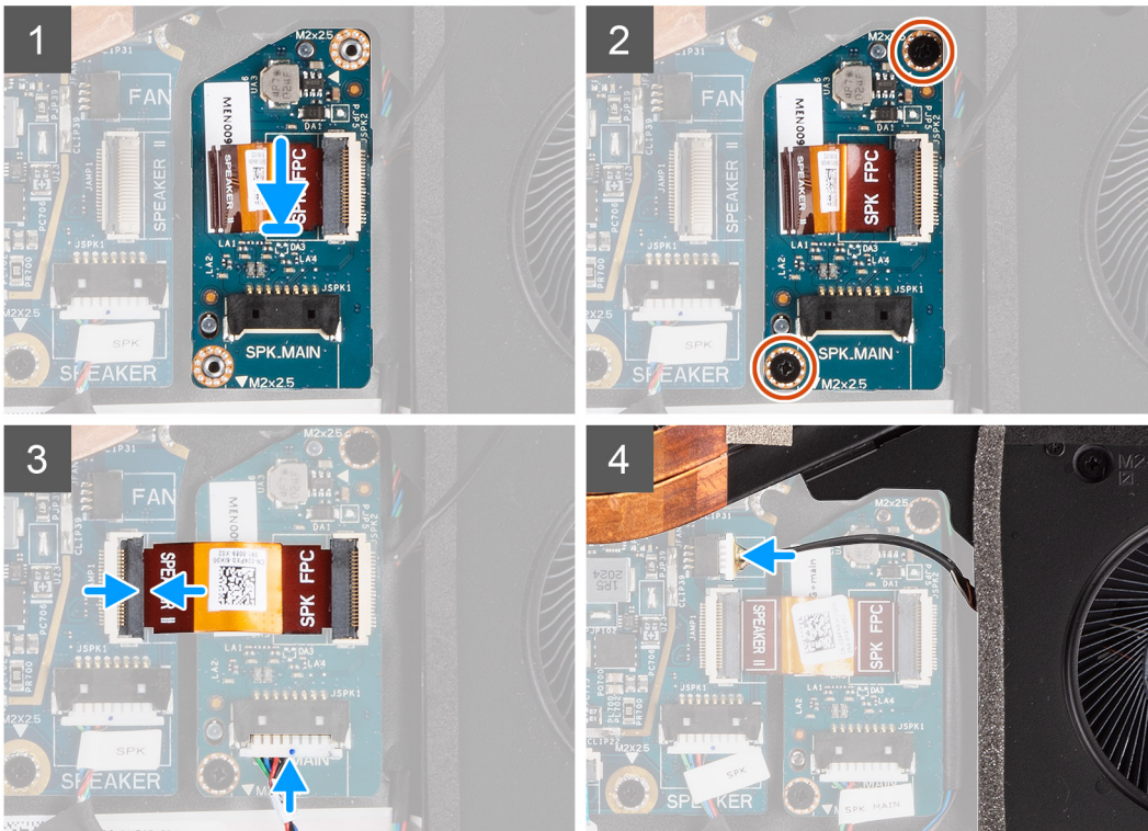
2x M2x2.5
