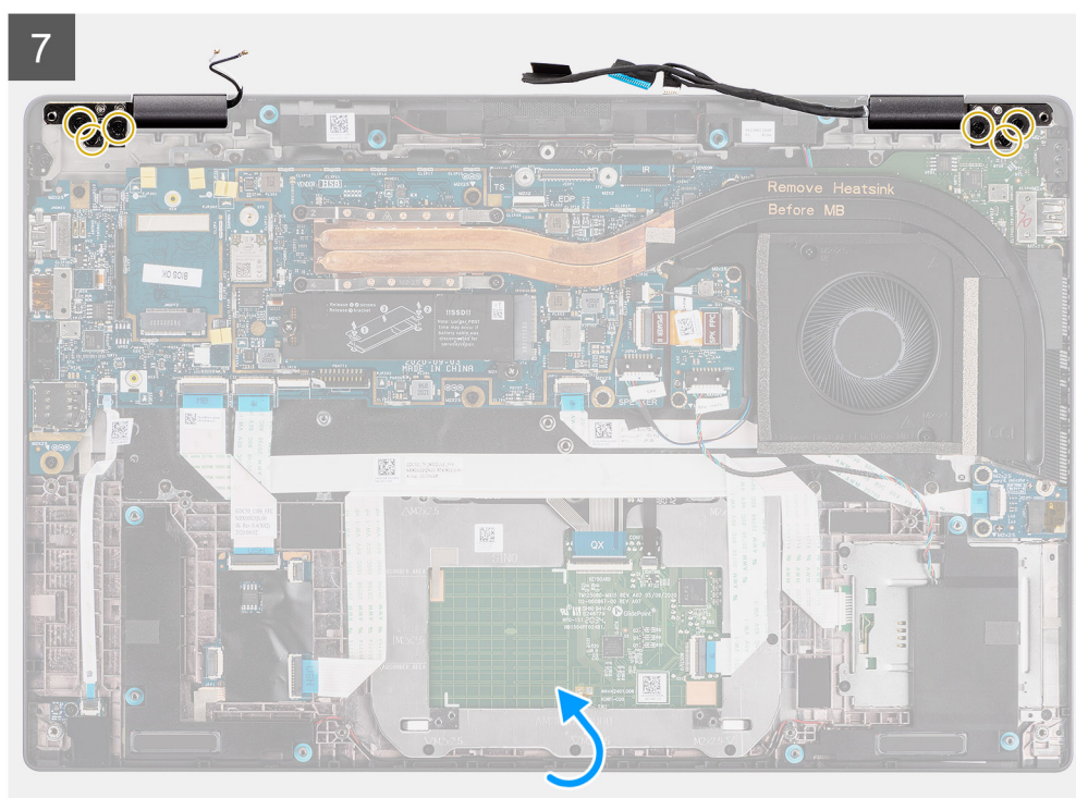
Figure 3. Display assembly with WLAN and WWAN antenna
