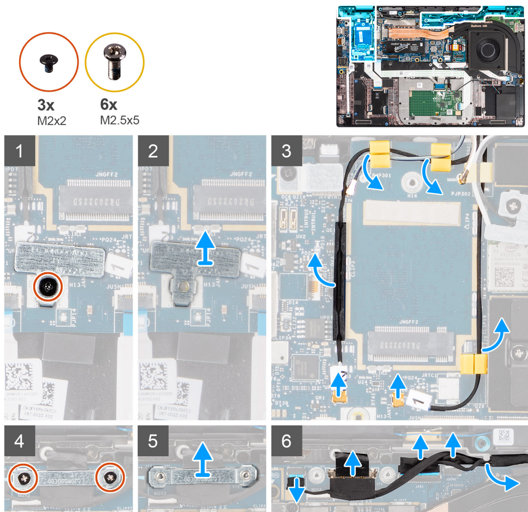
Figure 3. Display assembly with WLAN and WWAN antenna
