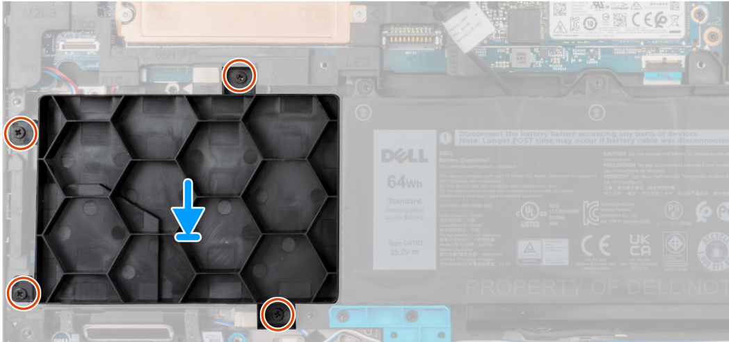
4x M2x4
