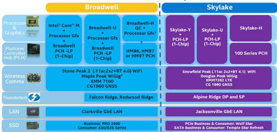
Figura 2. Roadmap tra Broadwell e Skylake
