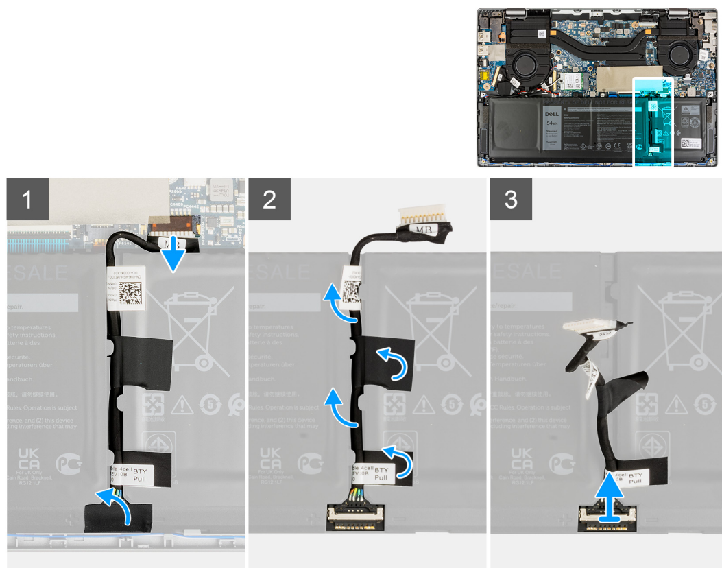
Figure 3. Removing the battery cable
