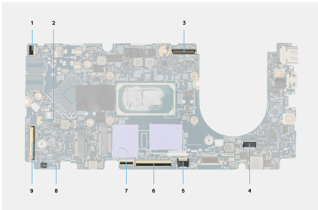
Figure 14. System-board connectors
