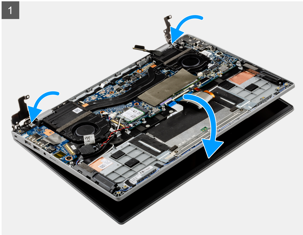
Figure 9. Installing the display assembly
