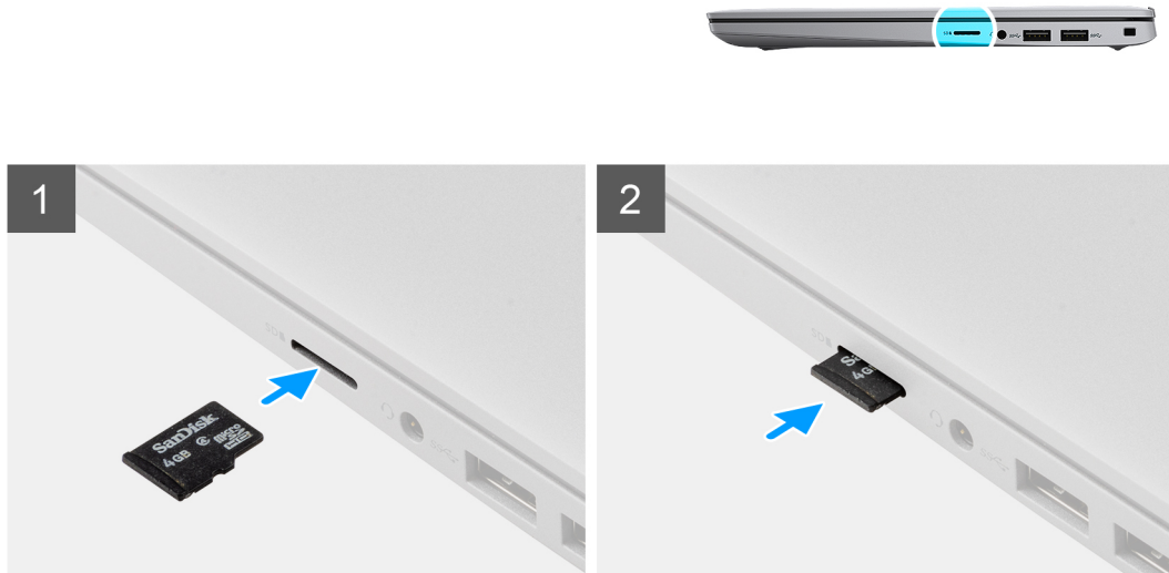
Figure 2. Installing the microSD-card
