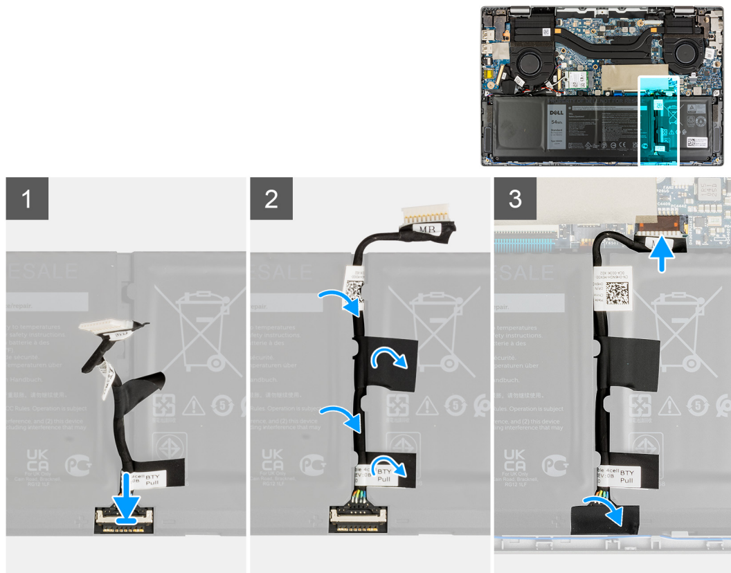
Figure 4. Installing the battery cable
