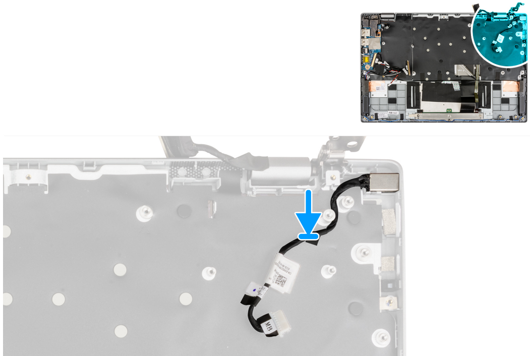
Figure 16. Installing the power adapter port
