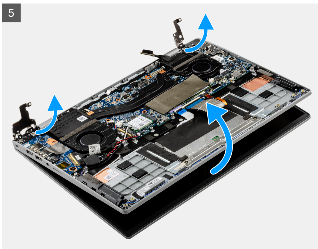
Figure 7. Removing display assembly
