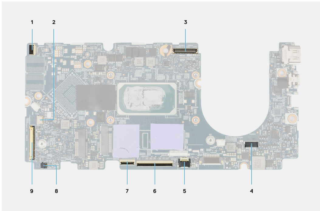
Figure 13. System-board connectors
