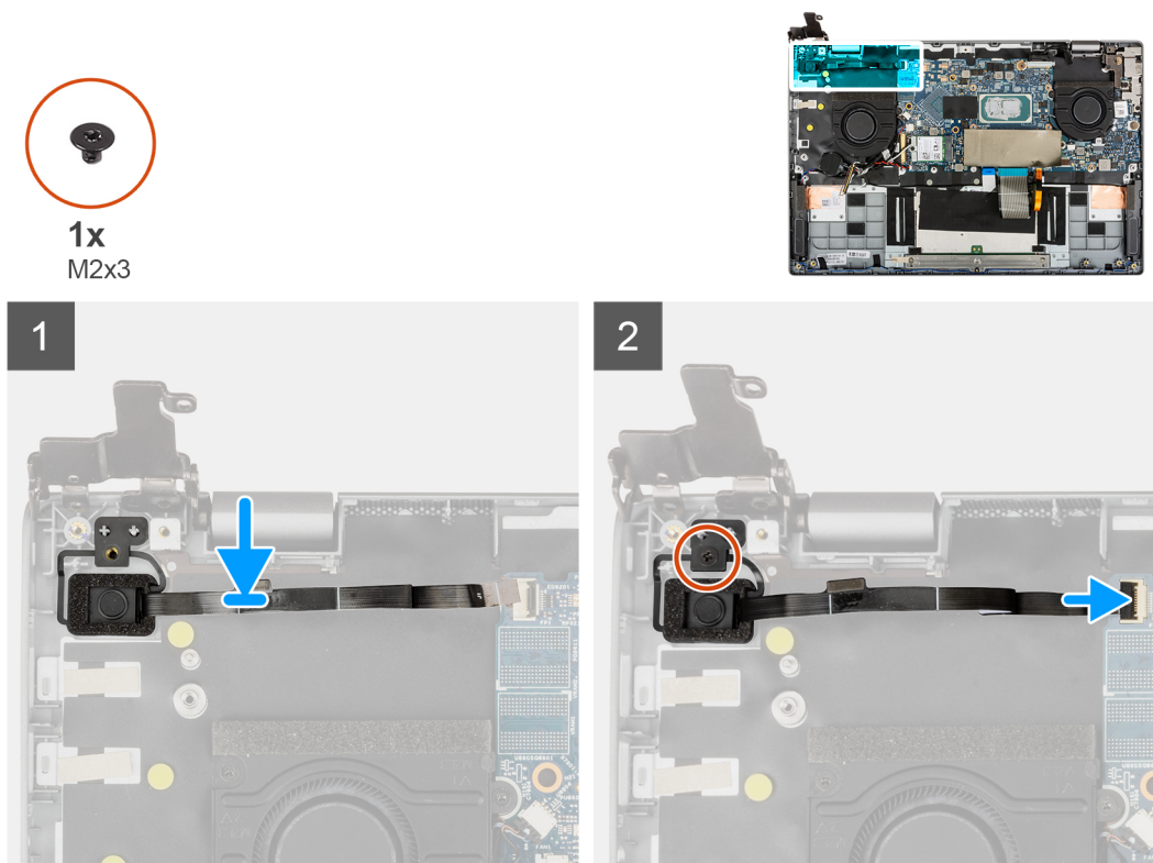
Figure 12. Installing the power-button board
