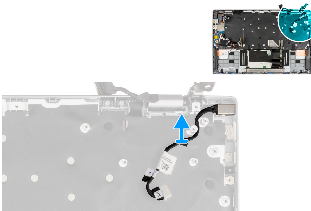
Figure 15. Removing the power adapter port
