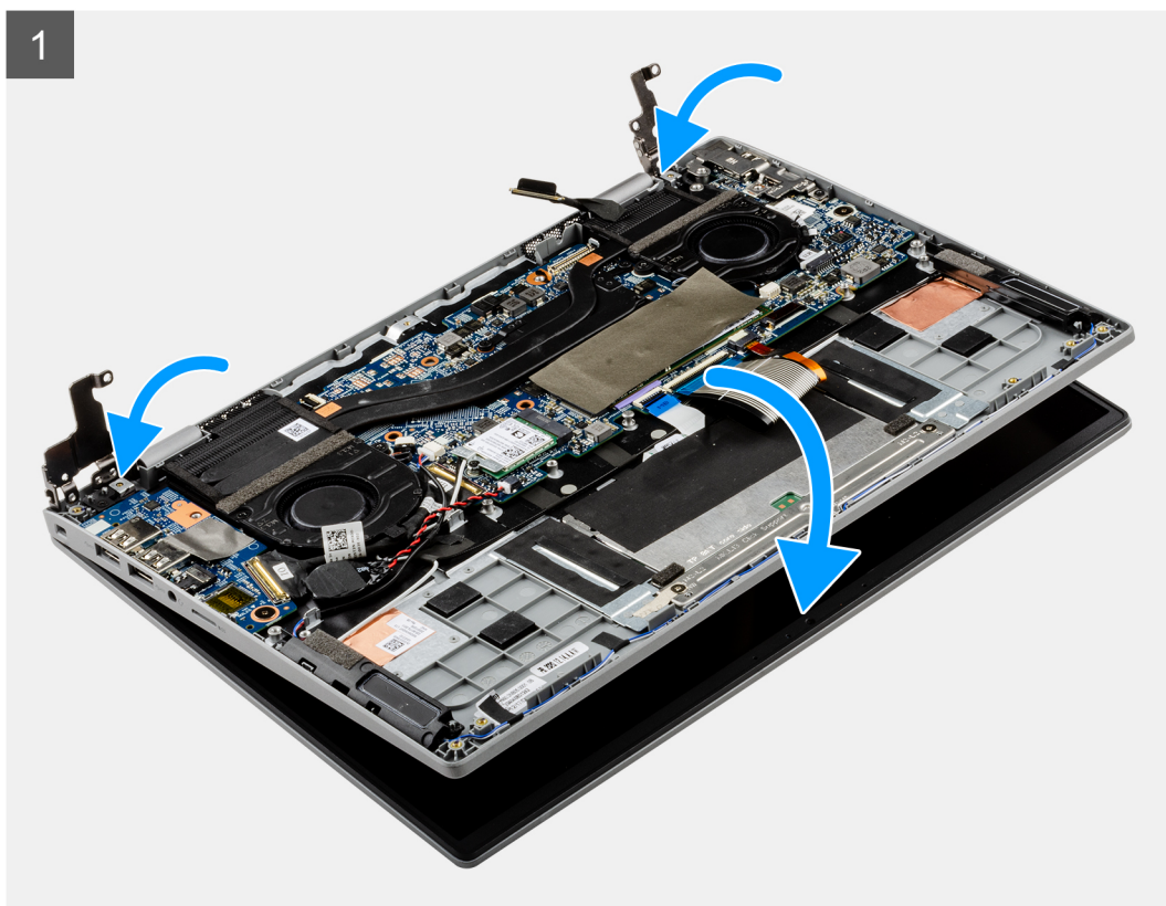
Figure 10. Place the display assembly
