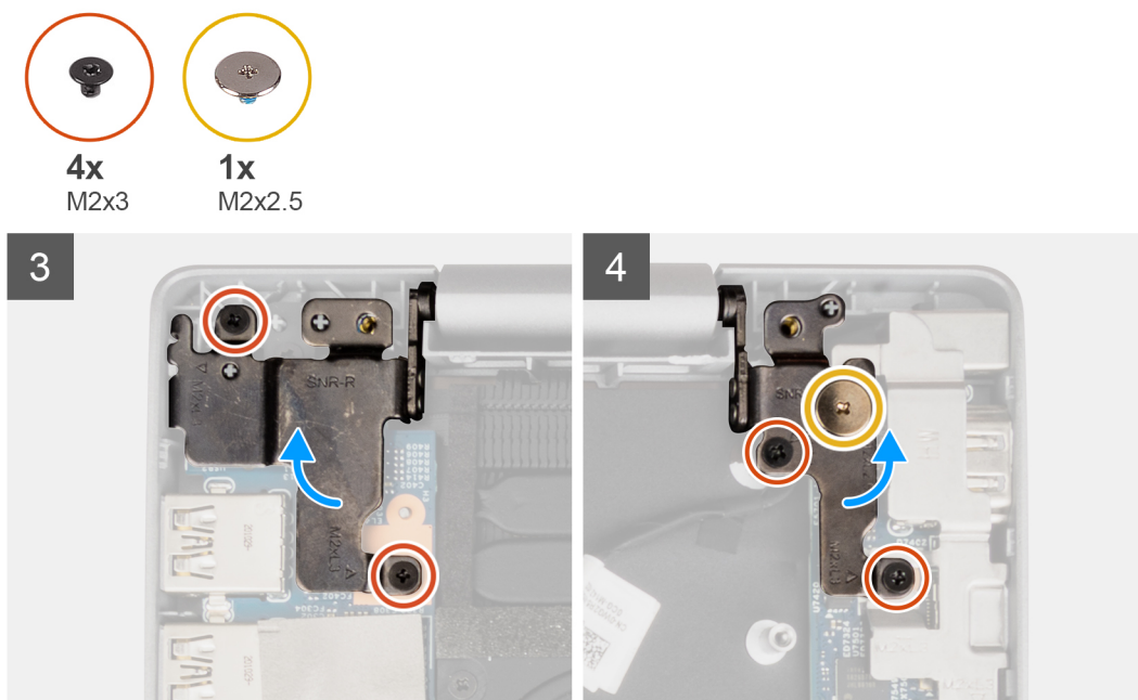
Figure 6. Removing the display assembly
