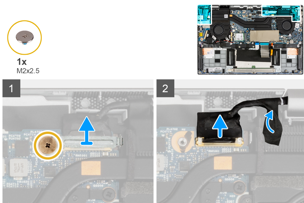
Figure 5. Removing the display assembly
