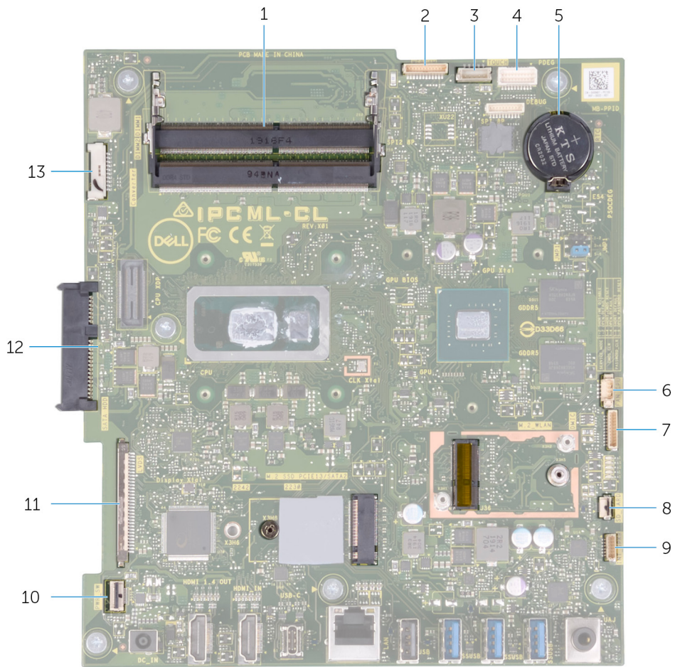
Figure 2. System-board connectors
