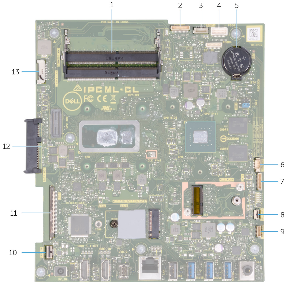
Figure 1. System-board connectors
