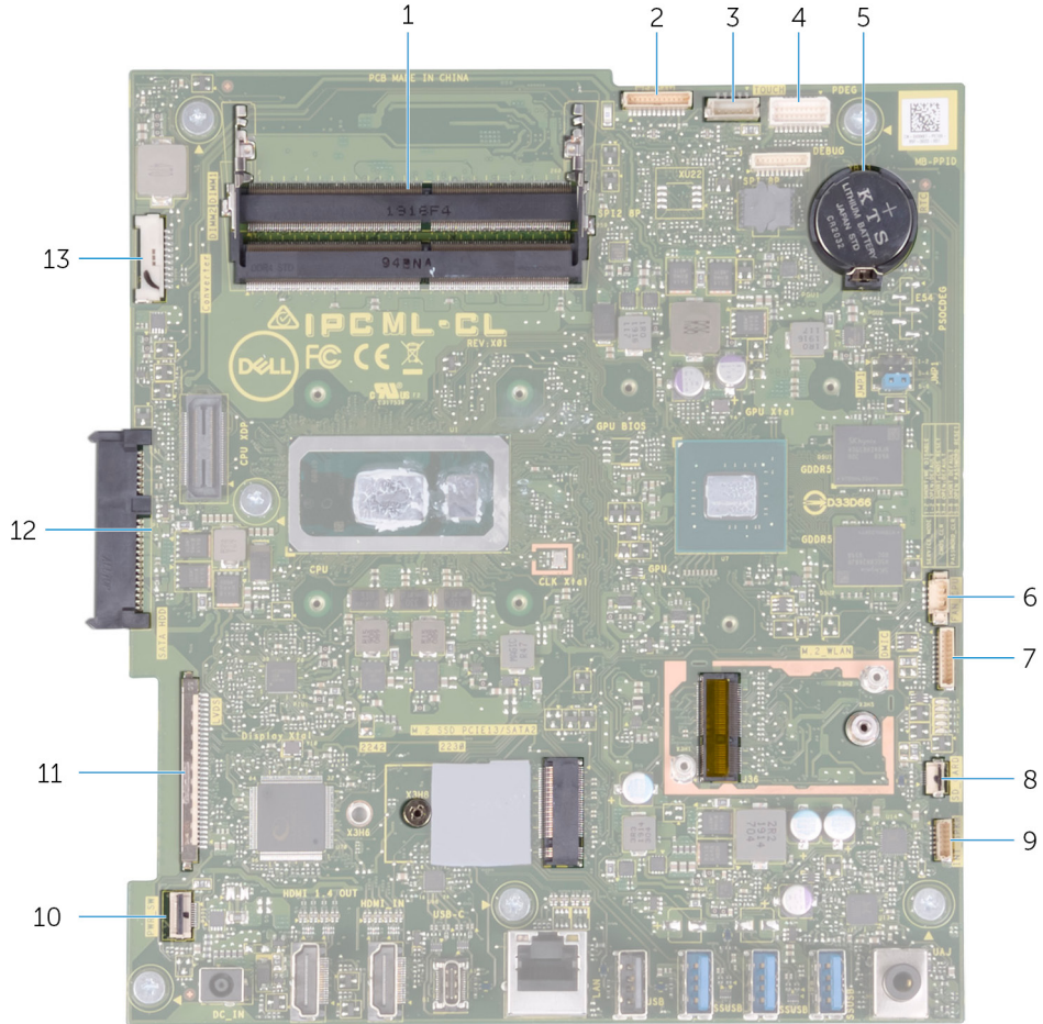
Figure 1. System-board connectors
