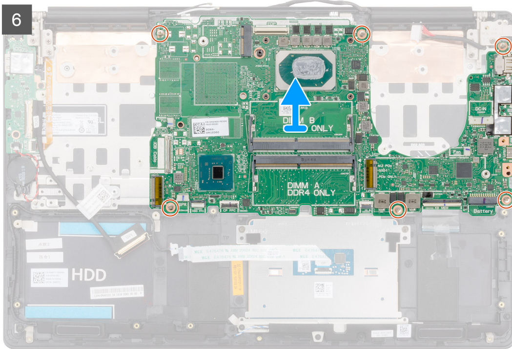
6x M2x4
