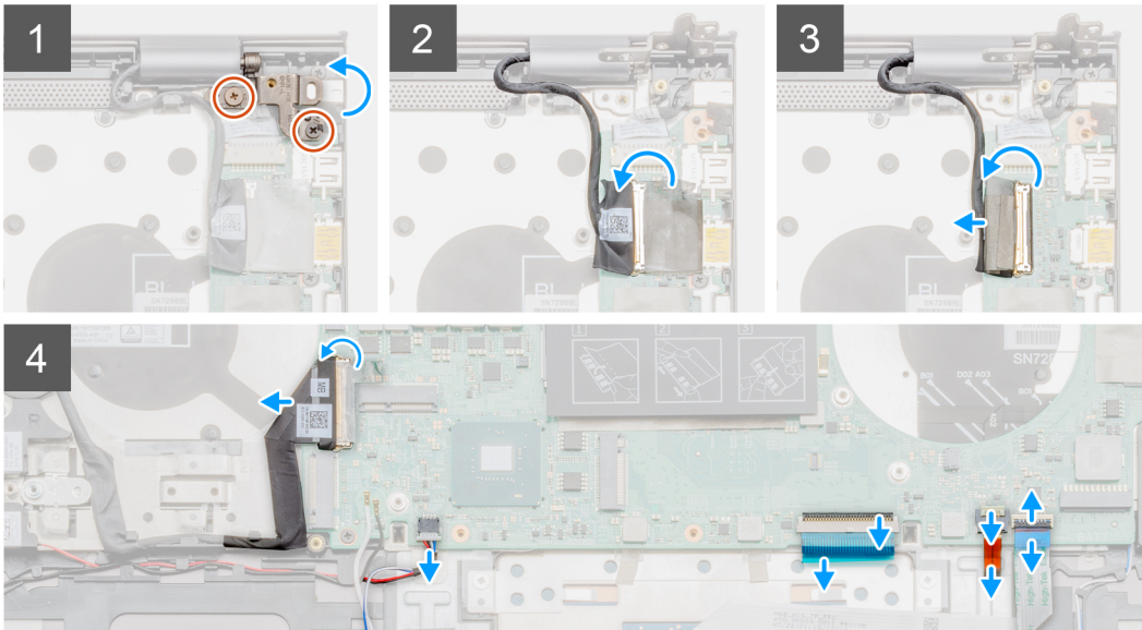
2x M2.5x5
