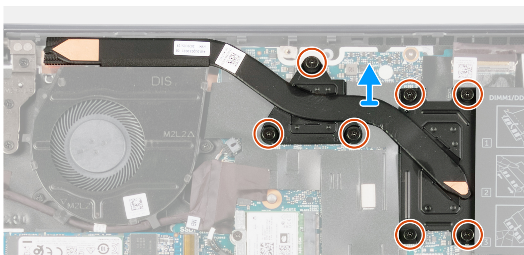
7x M2x5.85
