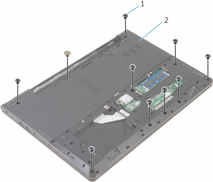
1 screws (10)
