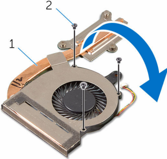
1 cooling assembly
