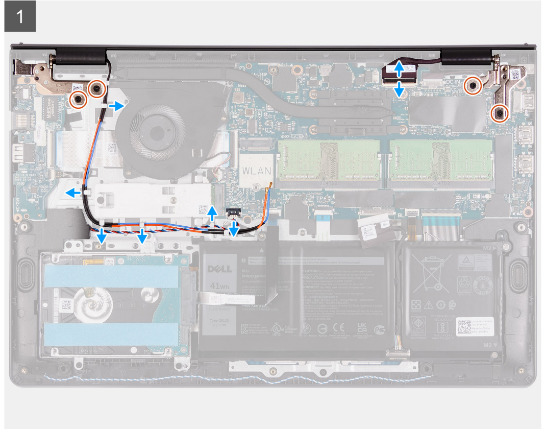
4x M2.5x5
