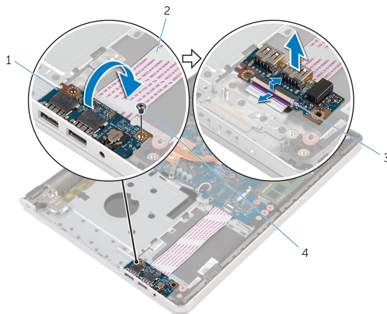
2. I/O-board cable
