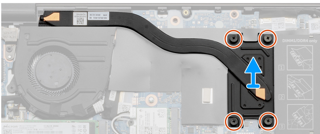
4x M2x5.85
