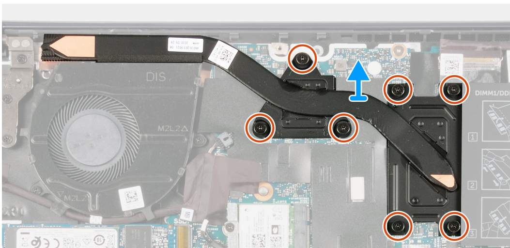
7x M2x5.85
