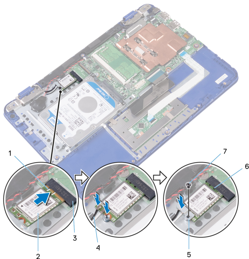
Figure 20. Replacing the wireless card
