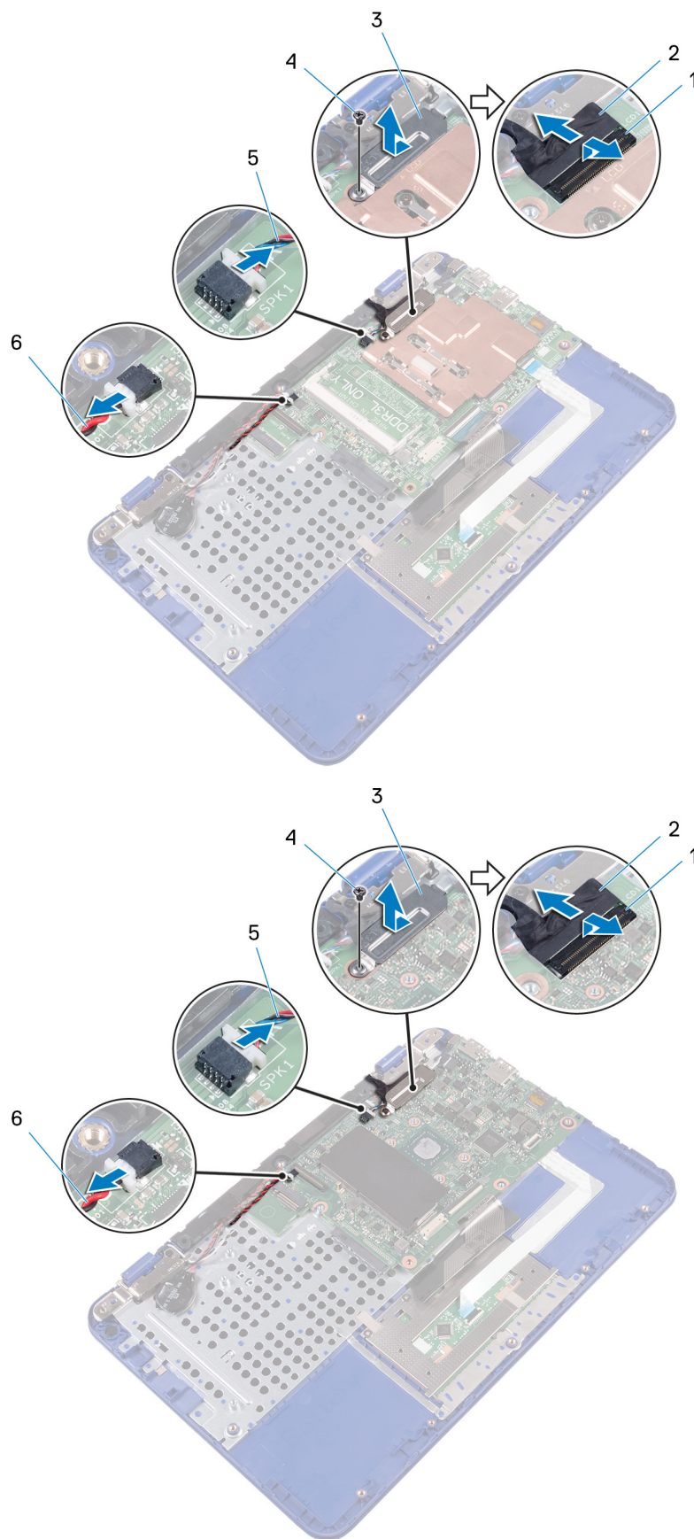
Figure 27. Removing the system board components
