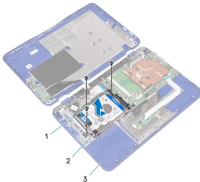
Figure 16. Removing the hard disc drive module
