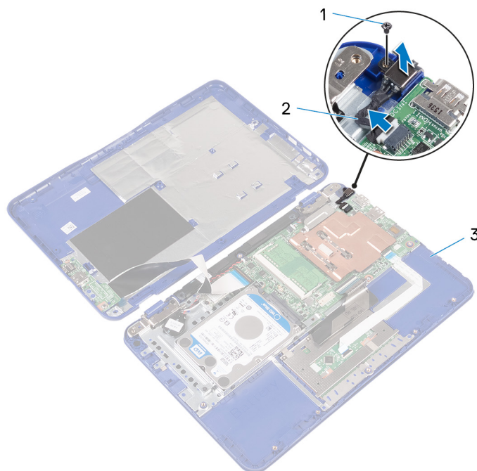
Figure 18. Removing the power-adapter port
