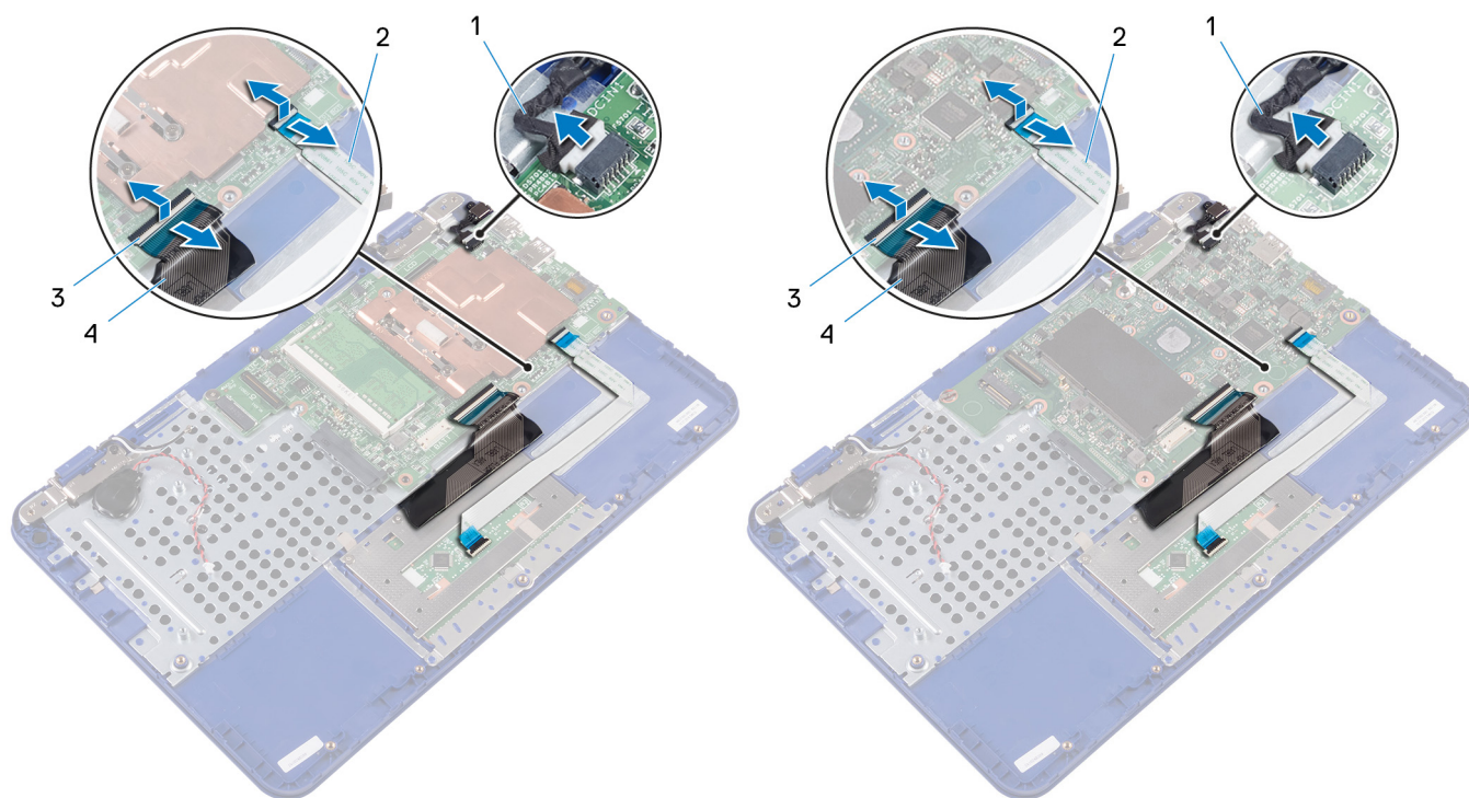
Figure 28. Removing the system board components
