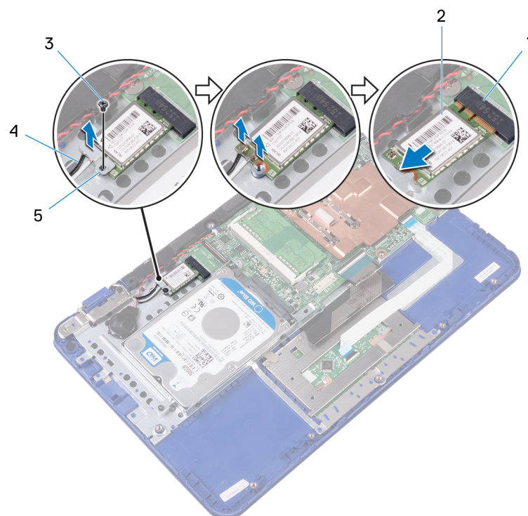
Figure 19. Removing the wireless card
