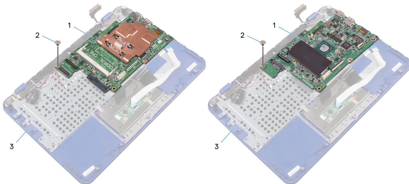
Figure 29. Removing the system board
