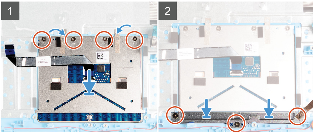
7x M2.x2
