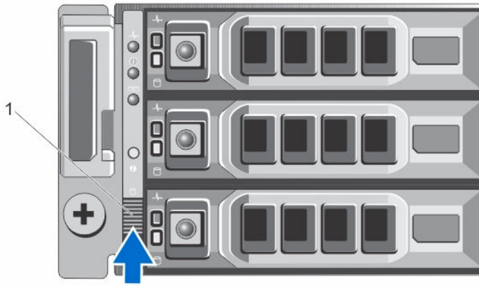
Figure 1. Setting the PowerVault MD1400 storage enclosure configuration switch
