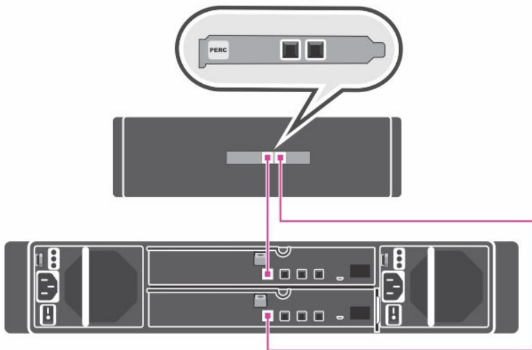
Figure 2. Connecting the DL4300 system to the MD1400 storage enclosure
