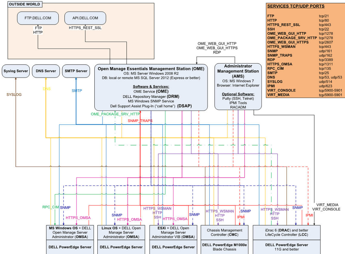
Figure 35. Network Connections
